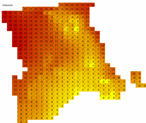
Figure 12: Reserves from the Gassum reservoir (GJ/m 2 ).
