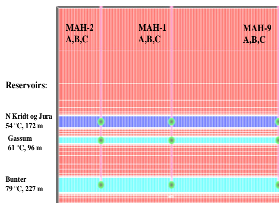
Figure 2: A vertical view of the 3 modeled reservoirs showing the reservoir gross-thickness
