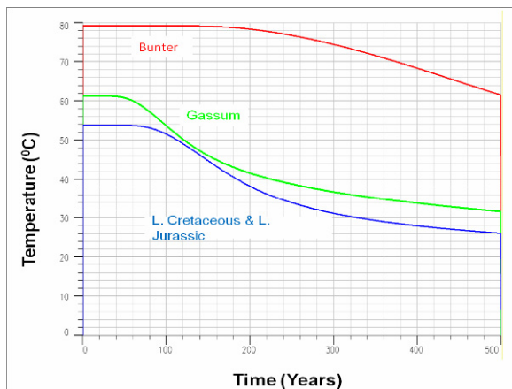
Figure 4: Production temperature decrease with time.
