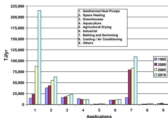
Figure 2. Comparison of worldwide energy in TJ/yr for 1995, 2000, 2005 and 2010.
