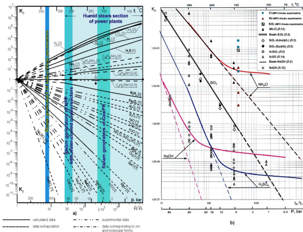
Figure 1: Radial diagram of balanced coefficients of inter-phase admixtures and gases distribution ( C_b ) between liquid and steam phases (a) and results of on-site investigations of C_b values for corrosion-aggressive admixtures (b).
