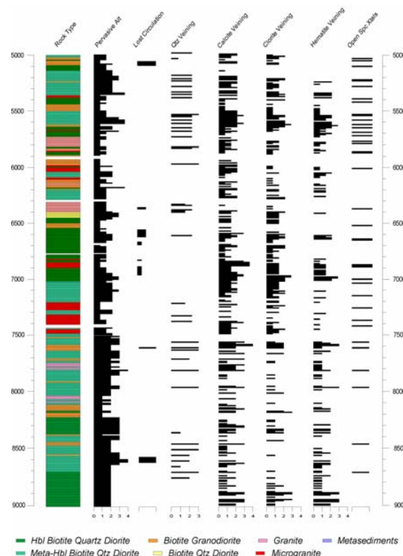
Figure 4. Summary of rock type and vein mineralogy as functions of depth for production well 38C-9.
