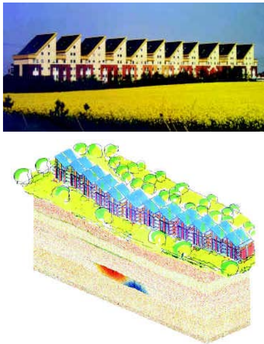
Figure 37: Row of residential houses in Rostock-Brinckmannshöhe, with location of ATES system (below) (photo and graphics: Aetna Energysysteme)
