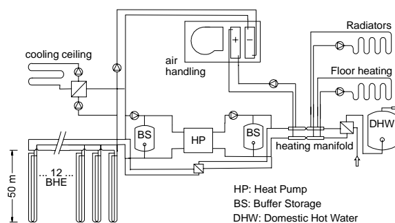
Figure 10: Umweltzentrum ("Environment Centre") Cottbus, view from outside and system schematic (photo Sanner)
