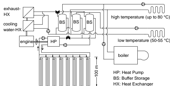
Figure 11: Office and shop "Naturwaren Maas", Gütersloh, view from outside and system schematic (photo EWS)
