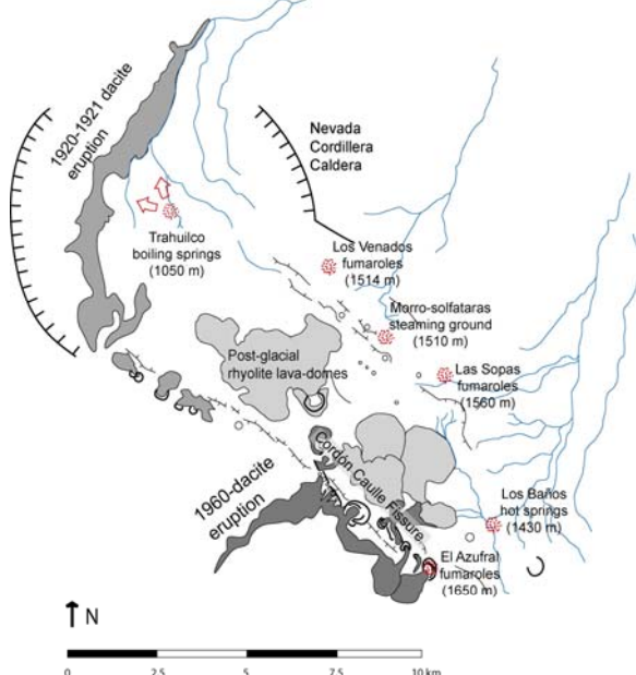
Figure 3: Localization of thermal manifestations of Córdón Caulle.
