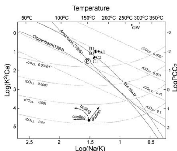
Figure 7: Na-K-Ca geoindicator applied to Trahuilco springs (after Giggenbach, 1988).
