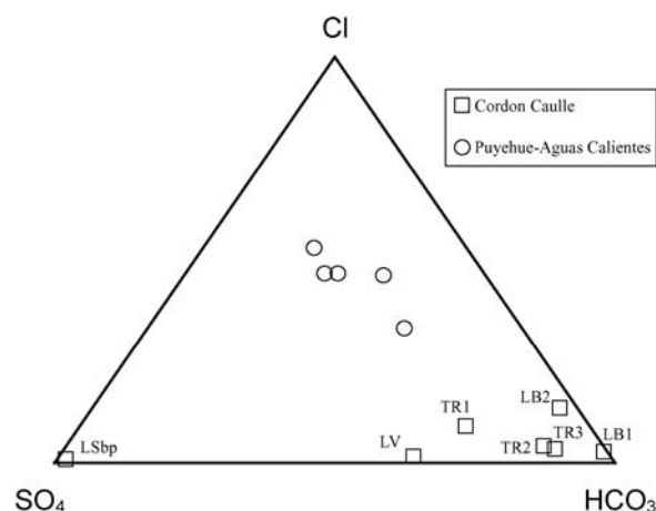
Figure 4: Cl-SO 4 -HCO 3 ternary diagram (Sepúlveda et al., 2004a). TR = Trahuilco hot spring; LV = Los Venados hot spring; LB = Los Baños hot spring; LShp = Las Sopas boiling pool (see Figure 3 for location).
