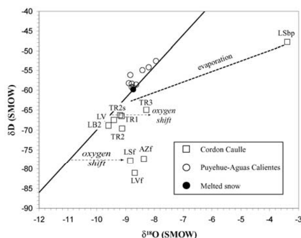
Figure 5: \delta\text{D} - \delta^{18}\text{O} plot applied to Puyehue-Aguas Calientes and Córdón Caulle. LSf, AZf and LVf = fumarole condensates (after Sepúlveda et al., 2004a).
