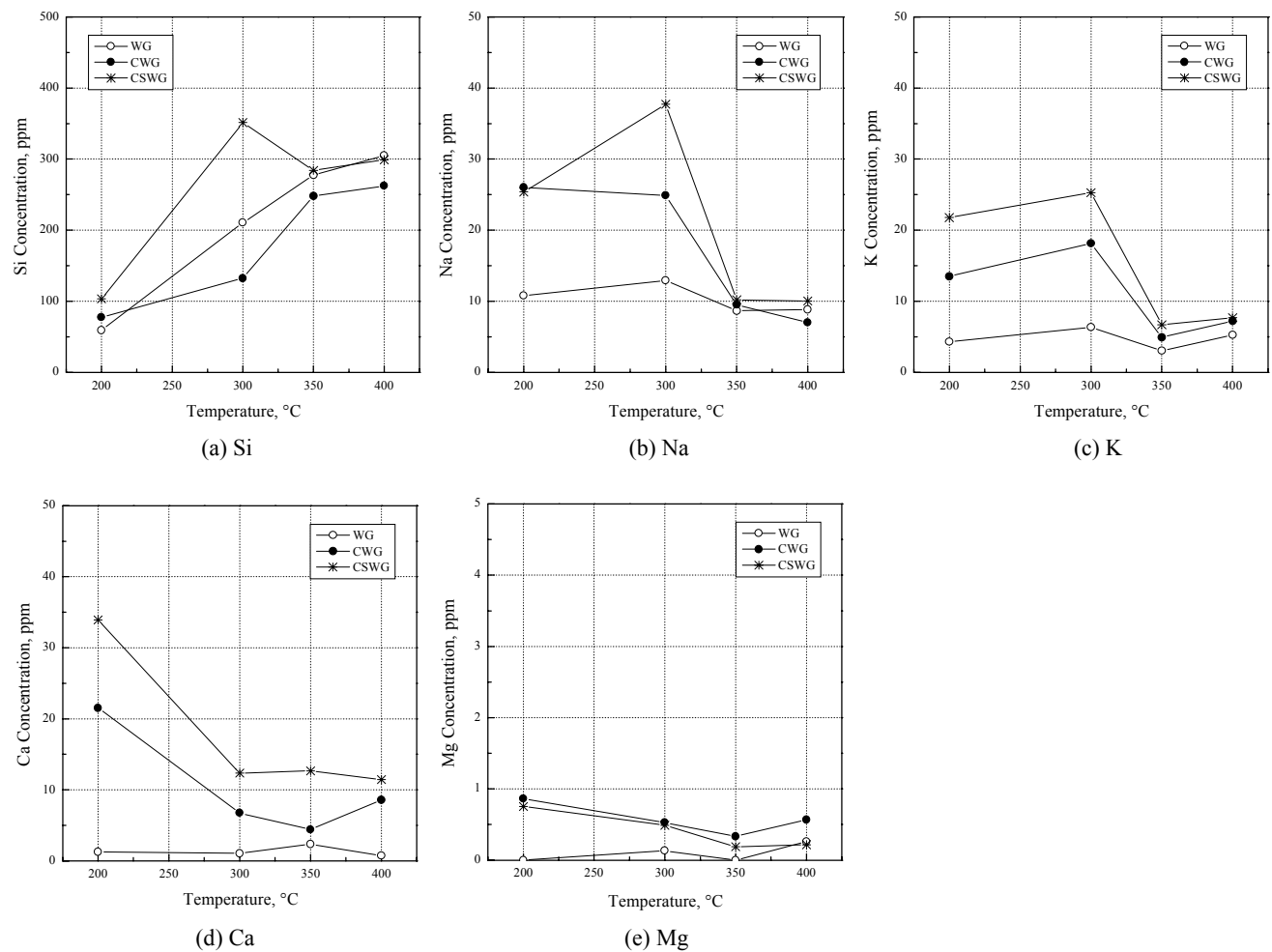
Fig. 6. Concentration of each element in solution measured by ICP after the experiments.
