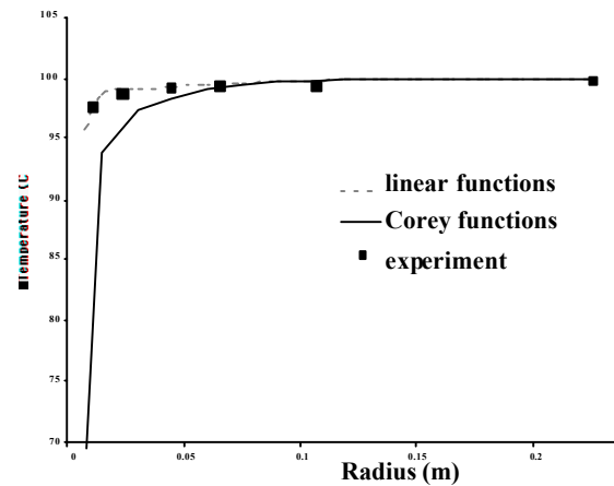
Figure 13: Fracture flow (temperature vs. radius) results from Wang and Horne (1999). Match using X-curves shown as dashed line, match using Corey curves shown as solid line.
