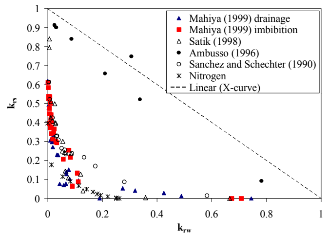
Figure 9: Comparison of results, k_{rs} vs. k_{rw} .
