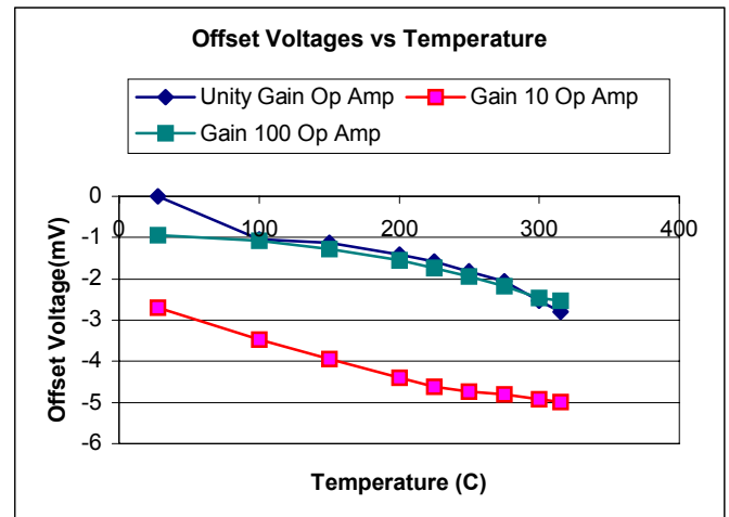
Figure 3. Several operational amplifiers were tested with three different gains, unity, X10, and X100. A) Shows the bandwidth of the amplifiers at 315°C. The unity gain bandwidth is over 100KHz. B) Shows the offset (DC Error) as a function of temperature.
