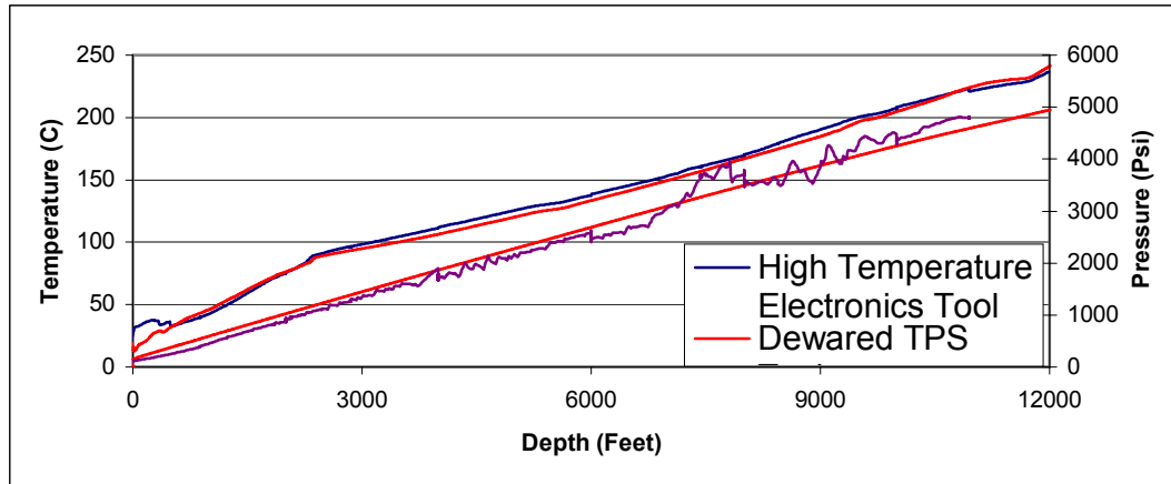
Figure 4. High-temperature tool operating without a heat-shielding flask (Dewar) is compared with the reading from a conventional Dewared logging tool. The temperature readings compare favorably while the pressure reads are tracking rising pressure but suffer from nonlinear increments. The next generation high-temperature tool will use a 12bit analog-to-digital converter for pressure measurement. This converter was not available at the time of the test. The new converter should greatly improve the pressure readings.
