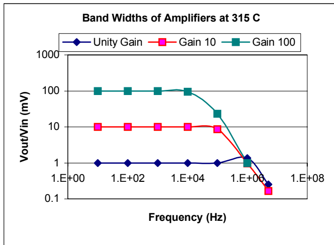
Figure 3. Several operational amplifiers were tested with three different gains, unity, X10, and X100. A) Shows the bandwidth of the amplifiers at 315°C. The unity gain bandwidth is over 100KHz. B) Shows the offset (DC Error) as a function of temperature.
