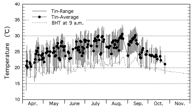
Fig. 12 Changes in inlet temperature of the observation DCHE and its bottom-hole temperature in the 1998 heat-charging season.
