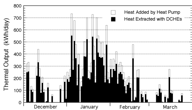
Fig. 9 Thermal output of the system in the 1997 snow-melting season.
