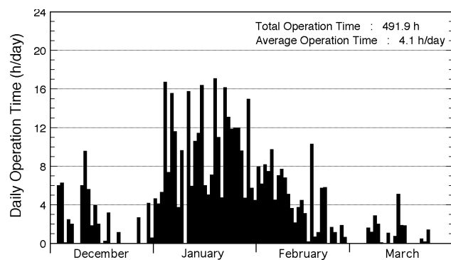
Fig. 6 Daily operation time of the system in the 1997 snow-melting season.
