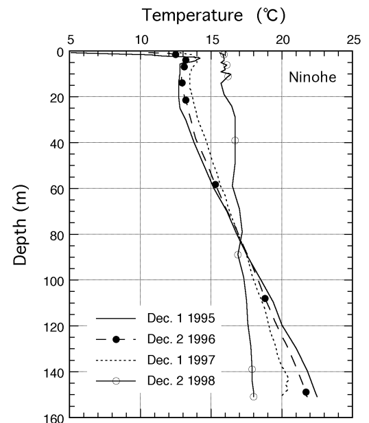
Fig. 15 Change in temperature profiles in the observation DCHE.
