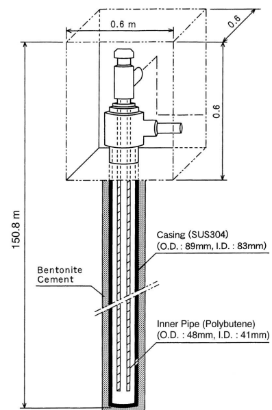
Fig. 2 Structure of the DCHE.
