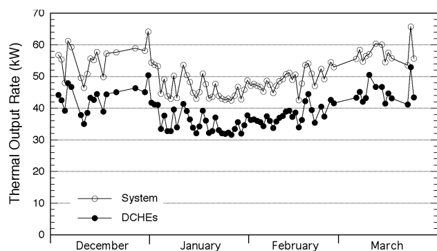
Fig. 10 Changes in thermal output rate of the system and DCHEs in the 1997 snow-melting season.
