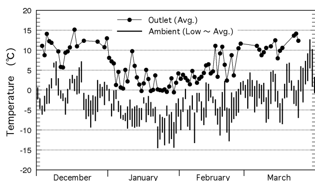
Fig. 7 Daily average outlet temperatures of the DCHE and ambient temperatures in the 1997 snow-melting season.
