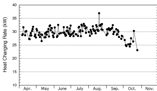
Fig. 13 Changes in heat charging rate in the 1998 heat-charging season.
