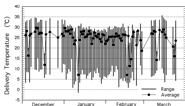
Fig. 8 Change in delivery temperatures in the 1997 snow-melting season.
