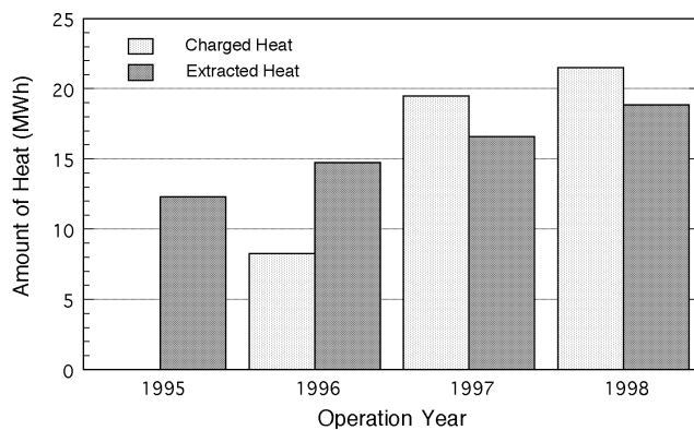
Fig. 14 Charged heat and extracted heat up to March 31, 1999. Operation year is from the first of April to the end of March in the next year.
