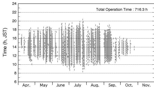
Fig. 11 Operation time of the system at Japanese Standard Time in the 1998 heat-charging season.
