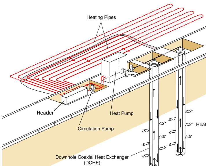
Fig. 1 Conceptual drawing of the Gaia Snow-Melting System.
