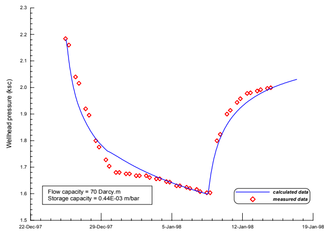
Figure 9. Measured and calculated wellhead pressure, Well 17-t
