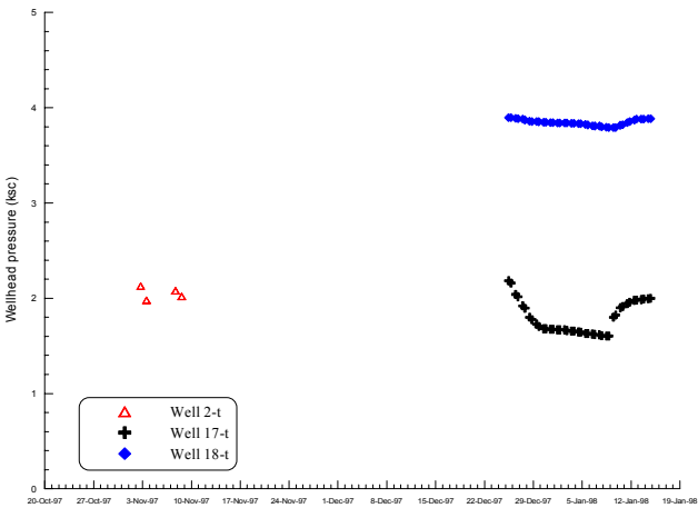
Figure 3. Flow test parameters versus time
