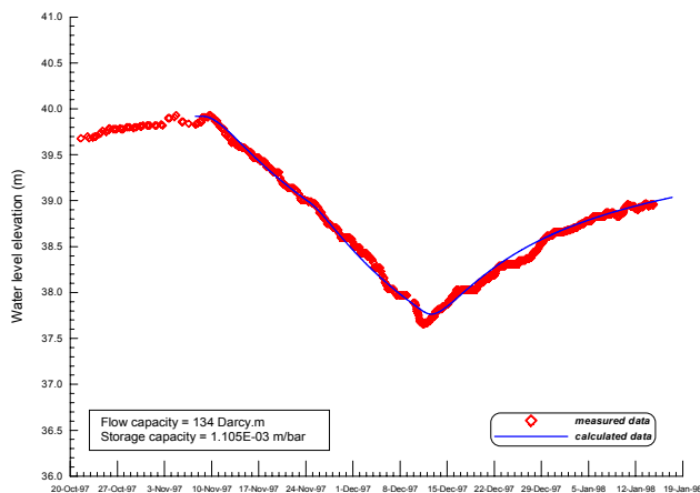
Figure 5. Measured and calculated water levels, Well 3-Zugdidi
