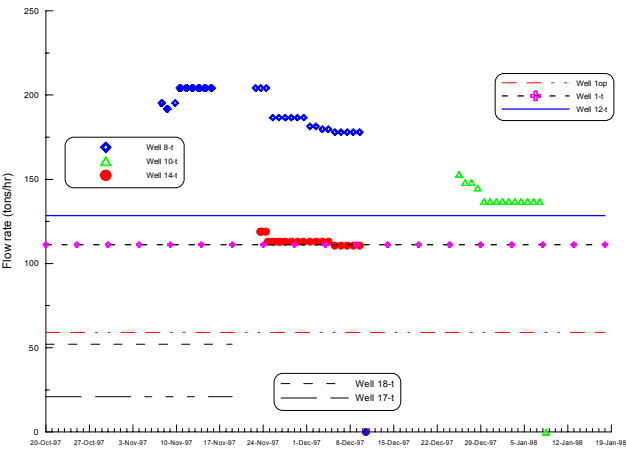
Figure 2. Flowrates of Zugdidi wells
