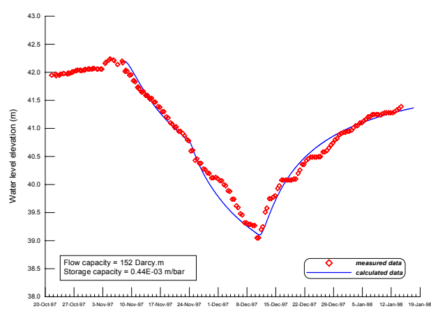
Figure 8. Measured and calculated water levels, Well 21-t
