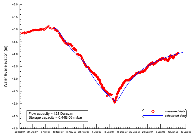
Figure 6. Measured and calculated water levels, Well 9-t
