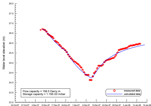
Figure 7. Measured and calculated water levels, Well 5-t
