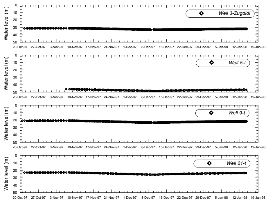
Figure 4. Water levels versus time
