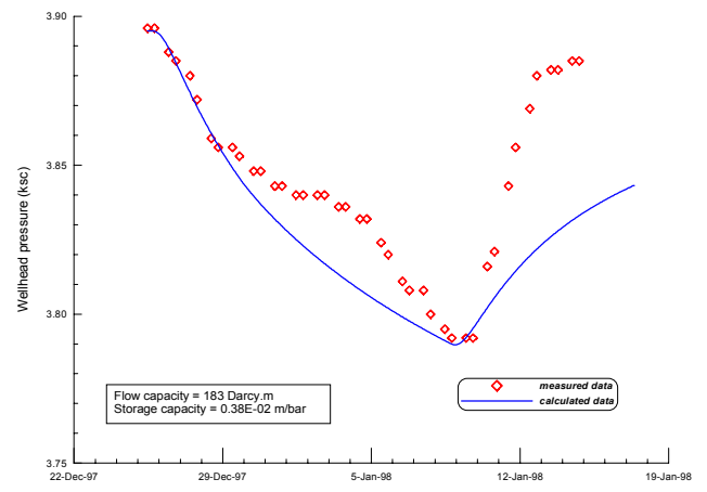
Figure 10. Measured and calculated wellhead pressures, Well 18-t
