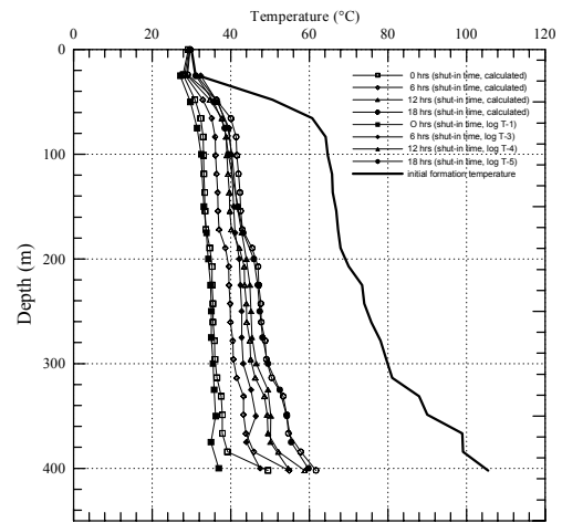
Fig. 6 Simulated and logged temperatures profiles in well LV-3 (at 400 m), Las Tres Virgenes Geothermal field.
