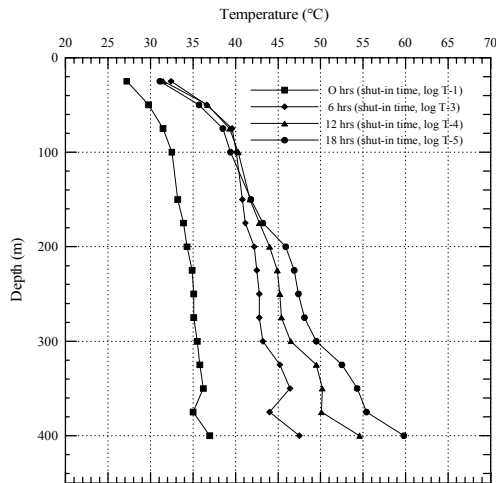
Fig. 4 Thermal behavior exhibited during the first drilling stage of well LV-3 at 400 m deep.
