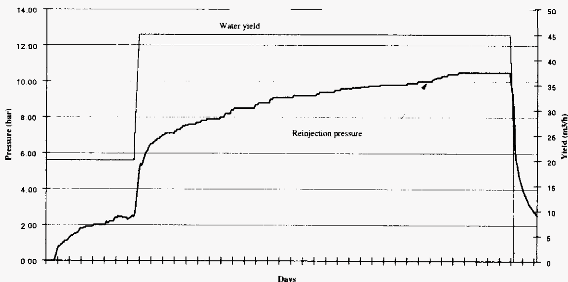
Figure 1 Reinjection pressure curve (Reinjection experiment in Szeged, 1992)
