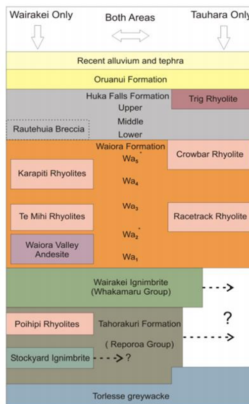
Figure 3: Stratigraphy of Wairakei-Tauhara geothermal system (Bignall et al., 2010).
