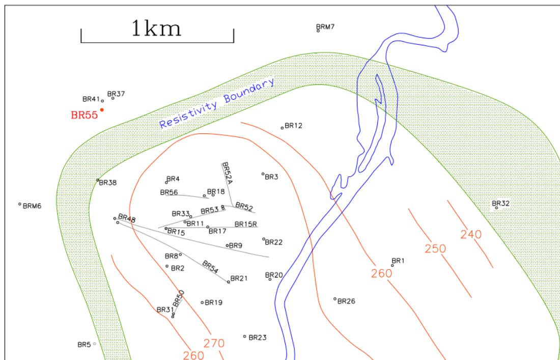
Figure 9: Map of well locations showing BR55 in the Northwest reinjection area beyond the Ohaaki Geothermal Field resistivity boundary (Bignall et al., 2007).
