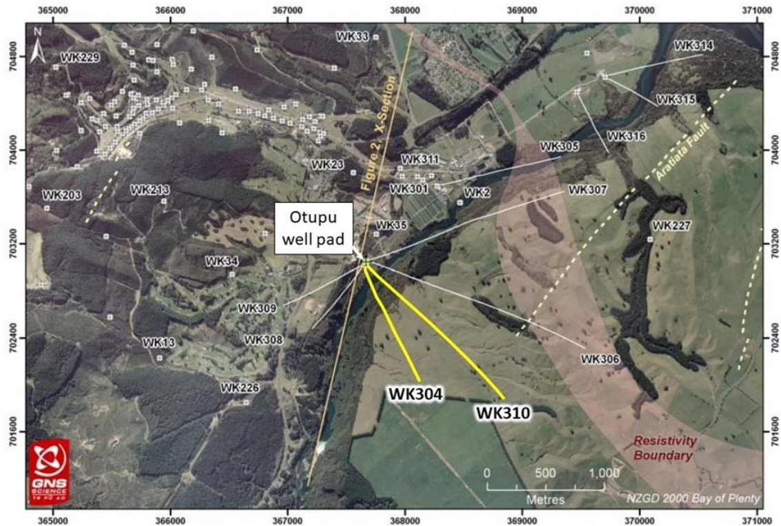
Figure 1: Aerial photo showing the location of Otupu reinjection well pad and radiating, deviated well tracks; WK310 and WK304 are highlighted. Modified from Milicich et al. (2010).
