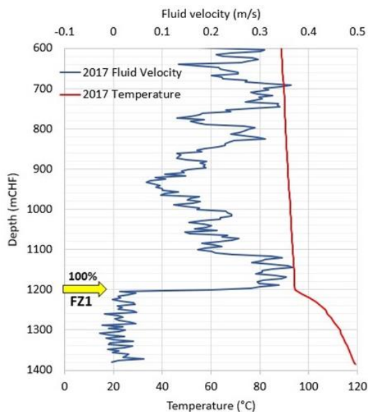
Figure 6: WK304 fluid velocity and temperature profiles at 23 t/h injection in 2017.
