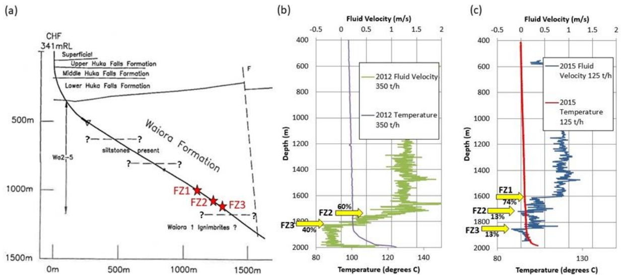
Figure 2: Feed zones of Table 1 indicated in: (a) geological cross-section along the line of WK310 (modified from original geology report in Wood, 1995); (b) 2012 fluid velocity and temperature profiles at 350 t/h injection; (c) 2015 fluid velocity and temperature profiles at 125 t/h injection.
