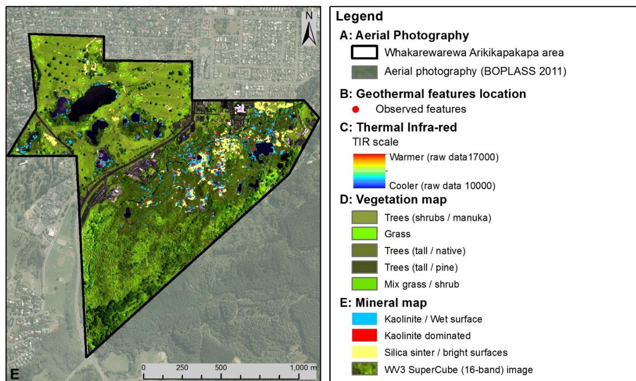
Figure 1. A. Aerial photograph of the Whakarewarewa-Arikikapakapa geothermal area, with significant features mentioned in the text labeled. B. Aerial photograph showing the distribution of geothermal features at Whakarewarewa-Arikikapakapa occurring in the GNS Science Geothermal and Groundwater Database. C. False colour TIR image of the raw TIR data for Whakarewarewa-Arikikapakapa. D. Vegetation map of Whakarewarewa-Arikikapakapa. E. Mineral map of Whakarewarewa-Arikikapakapa.
