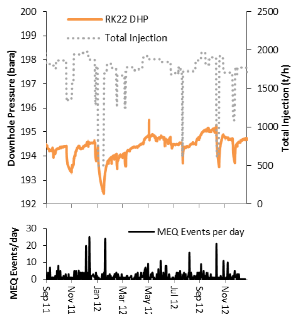
Figure 6: Comparison of MEQ events per day to downhole pressure monitoring in RK22 and total deep injection. Two swarms, in January and October, 2012 appear to be associated with transient pressure change in the injection area. Other swarms however do not appear to have a correlation with pressure change in the injection area.
