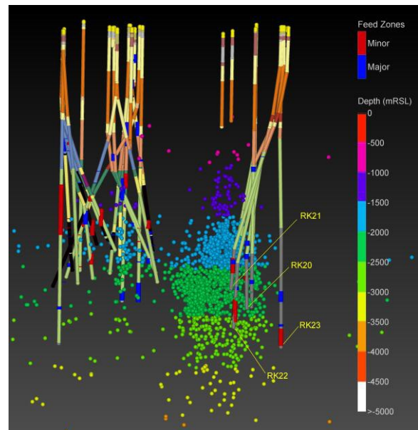
Figure 9: MEQ with depth in relation to injection feedzones (blue and red bars on well tracks). The majority of MEQ activity has been at the same depths as injection feedzones (-1500 m to -3000 m). Relatively few events have occurred below the injection feeds and from this, vertical permeability in the injection area is inferred to be relatively low.
