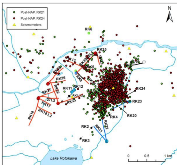
Figure 4: MEQ locations from February, 2010 to December 2012. A shift in the location of MEQ activity to the northwest is coincident with a large shift of injection from RK21 into RK24.
