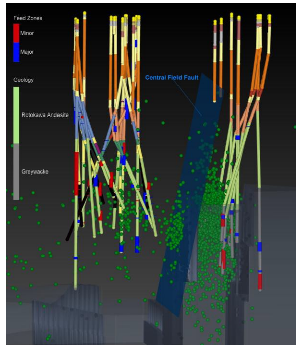
Figure 7: MEQ's from July, 2008 to December, 2012, the Central Field Fault and greywacke. Vertical offset in the greywacke from the injection area to the production area is ~500m depth.
