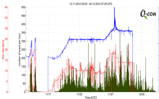
Figure 6: Injection pressure, flow rate and seismicity data for the extended stimulation
