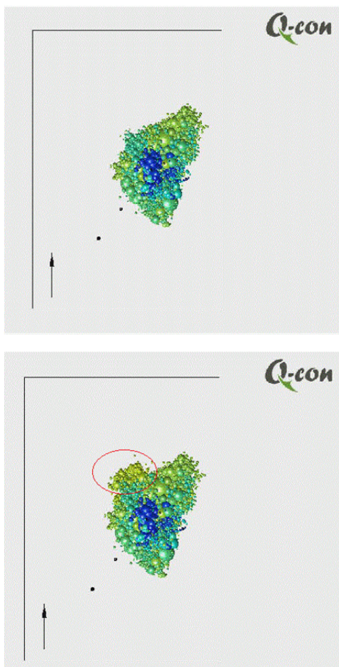
Figure 9: Seismicity from 2012 Habanero 4 stimulation showing temporary barriers. Top picture includes seismicity from 14/11/12 to 23/11/12. Bottom picture includes seismicity from 14/11/12 to 24/11/12.
