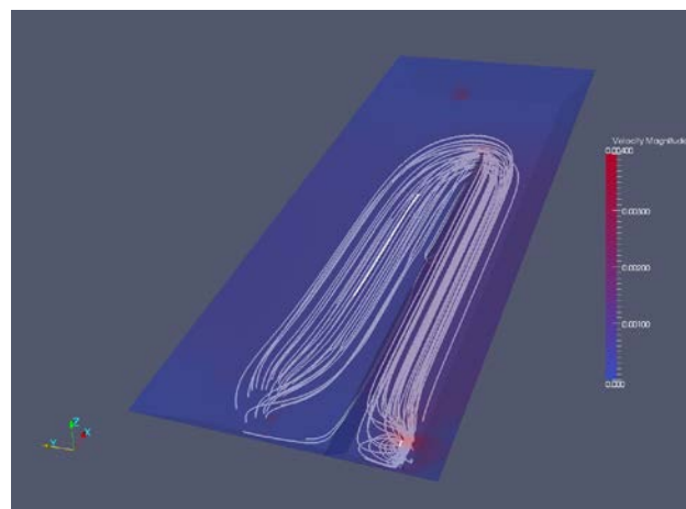
Figure 5: Hydraulics of street layout
