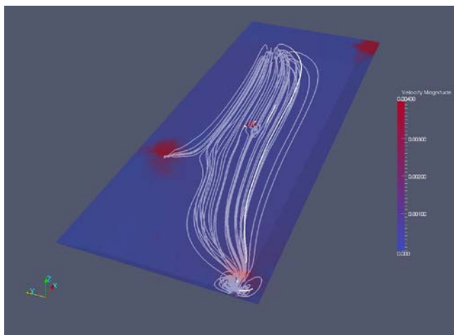
Figure 3: Hydraulics of the Basic Pond
