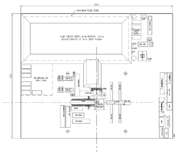
Figure 1: 'Typical' Rig Layout
