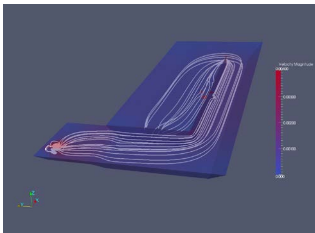
Figure 6: Hydraulics of Ideal layout
