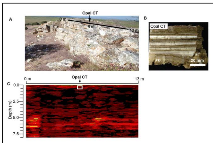
Figure 7: Trace element-rich opal-CT outcrop at Opal Mound, Utah, USA. (A) Site photograph of opal-CT sinter and the location of the 13 m GPR profile. (B) Hand specimen of opal-CT sinter. (C) GPR image, taken at where the sinter outcrops along the 13 m GPR transect line, shows strong continuous horizontal near-surface reflections (red areas) and the subsurface fractures are captured and shown as black areas.
