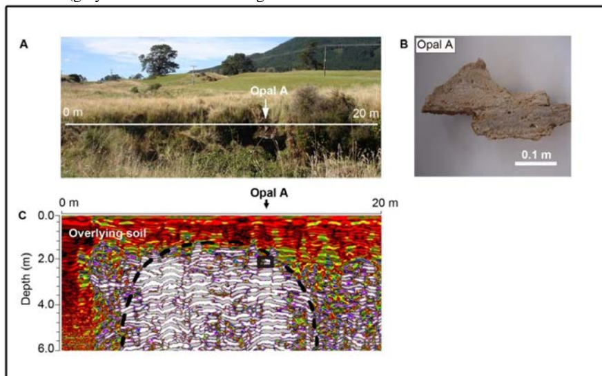
Figure 2: Trace element-poor sinter with opal-A silica phase and corresponding hand specimen and GPR image located at Horohoro, New Zealand. (A) Site photo of opal-A sinter outcrop and the 20 m GPR transect line which extends over the outcrop. Arrow showing the location of hand specimen collected. (B) Photograph of hand specimen of opal-A sinter sampled. (C) GPR image collected over outcrop. The grey and white coloured reflections indicate sinter at depth while the red and yellow reflections indicate overlying soil. The black box marks the location of the sinter sample collected and the dotted line shows the approximate boundary of the buried sinter (~12 m long x 4 m thick).
