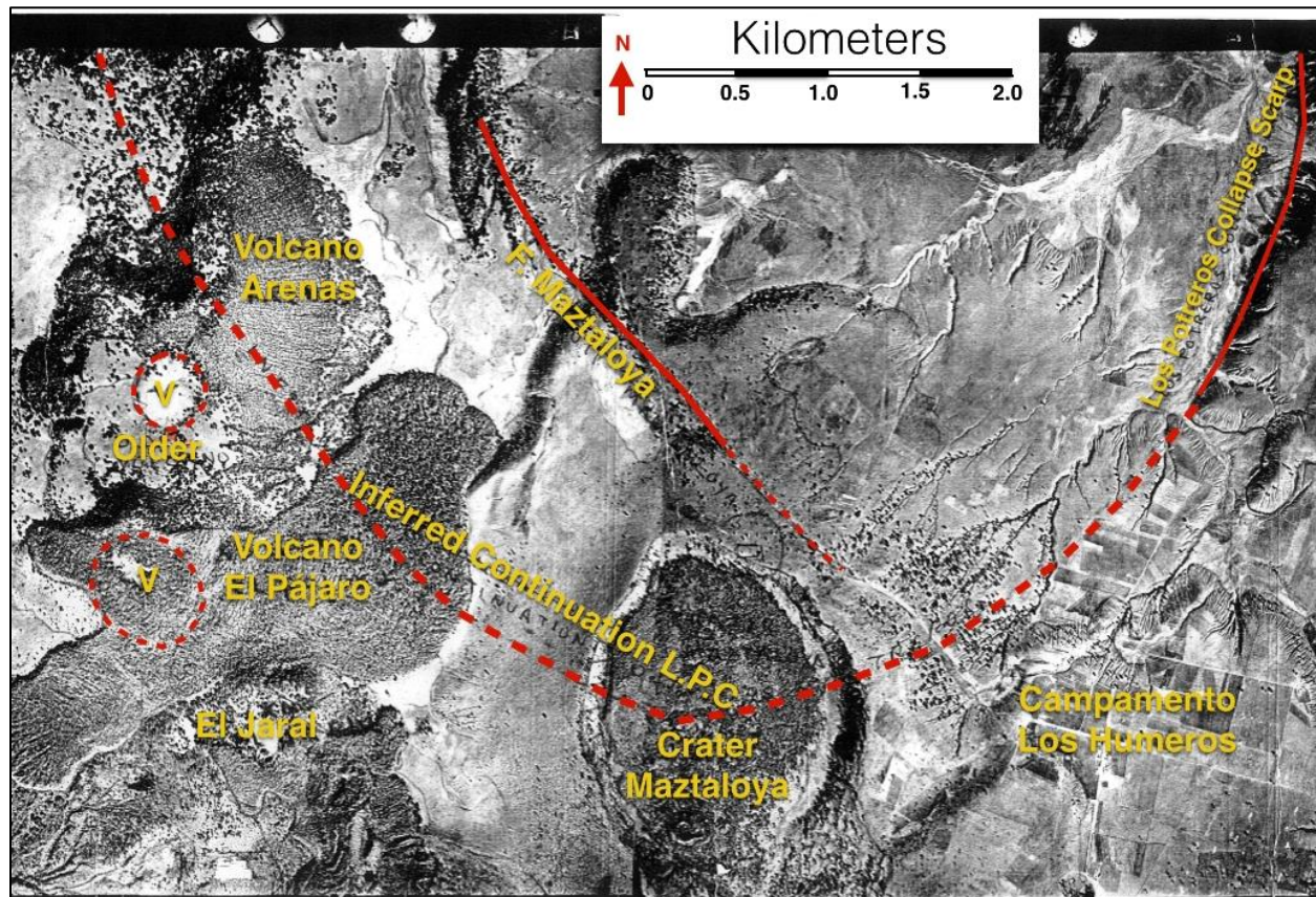
Figure 3. The Maztaloya crater, located at the southern rim of the LPC, and the Maztaloya normal fault.
