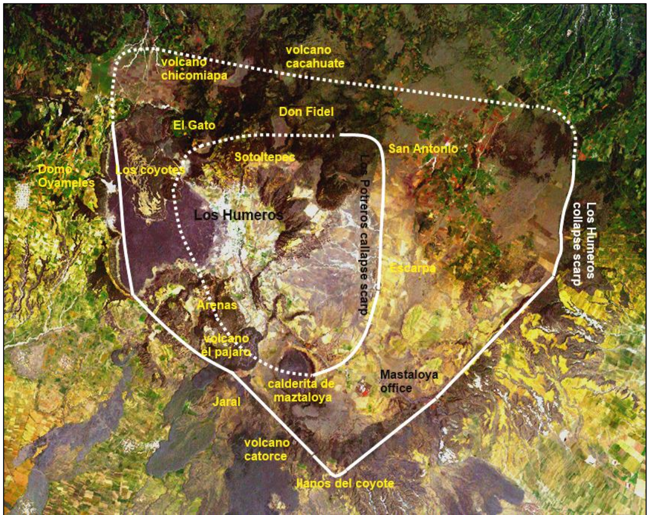
Figure 5. The new proposed rims of the Los Humeros and Los Potreros calderas.
