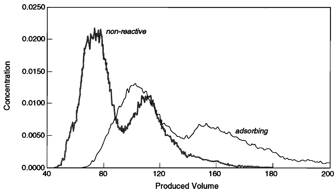
Figure 5. A comparison of non-reactive and adsorbing tracers at 10 years.
