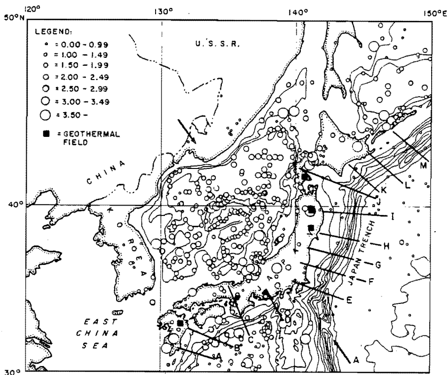
Figure 2 - Heat flow in Japan and vicinity in relation to the location of geothermal fields and transverse zones. Basic heat flow map from Watanabe et al (1977). Locations of geothermal fields (filled squares) from Nakamura. Transverse zones A-L as in Figure 1. Zones L and M outline a block which ruptured in 1973 and ruptured earlier in 1894.
