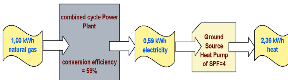
Figure 1: Primary energy converted to useful heat by GSHP
