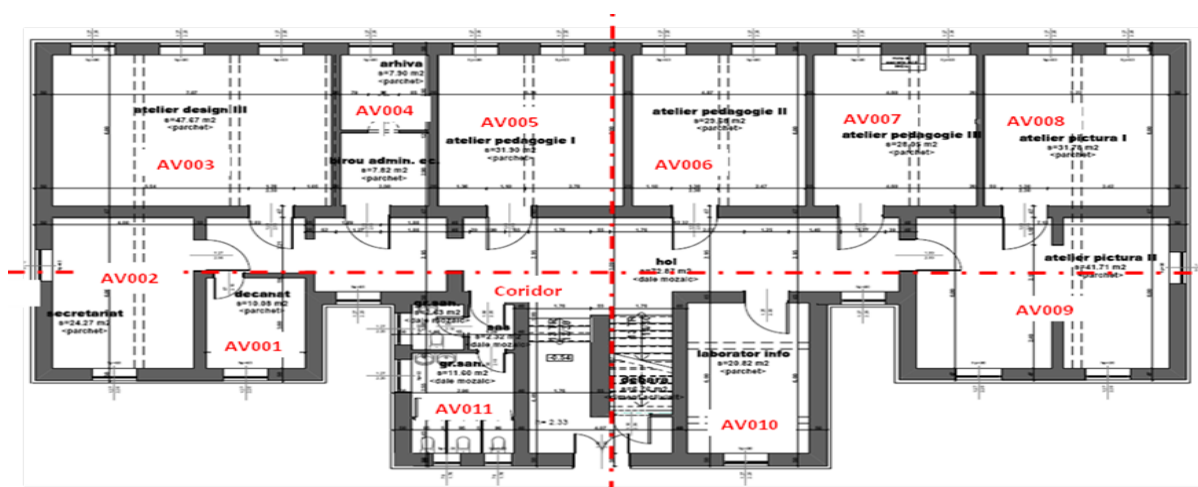
Figure 5: Geometrical characteristics of the ground floor of Visual Arts building
