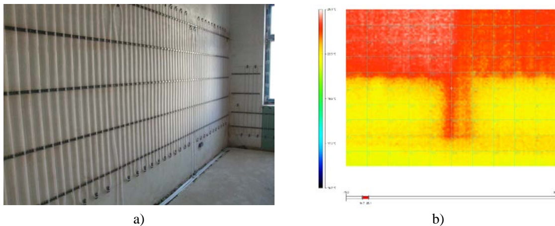
Figure 7: Heating/cooling wall pipes
