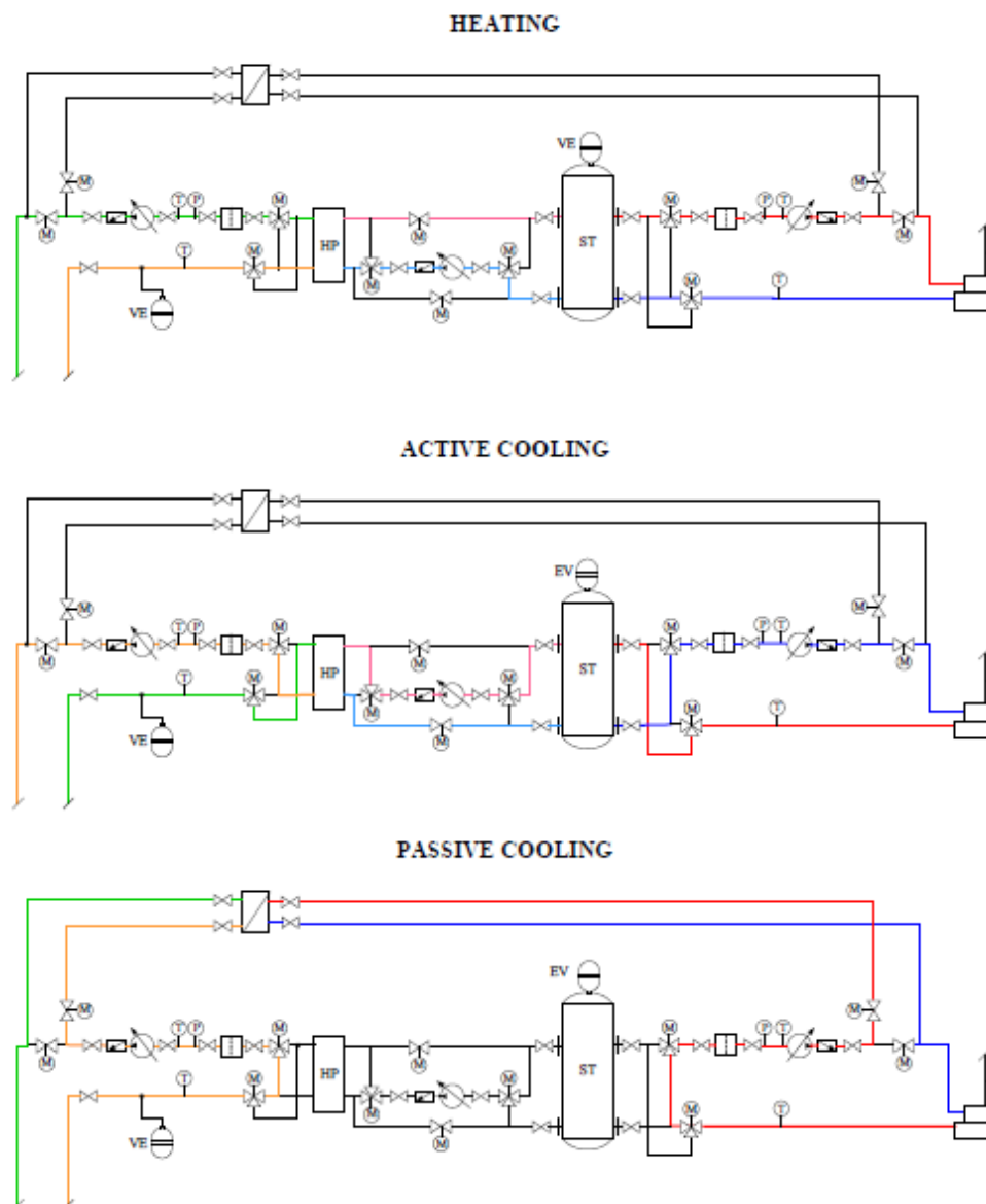
Figure 11 – The hydraulic layout out of Ground-Med Oradea demo-site
