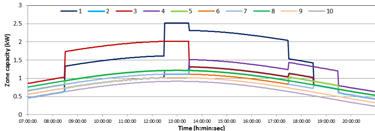
Figure 3: Zone load profile between 7 am – 9 pm
