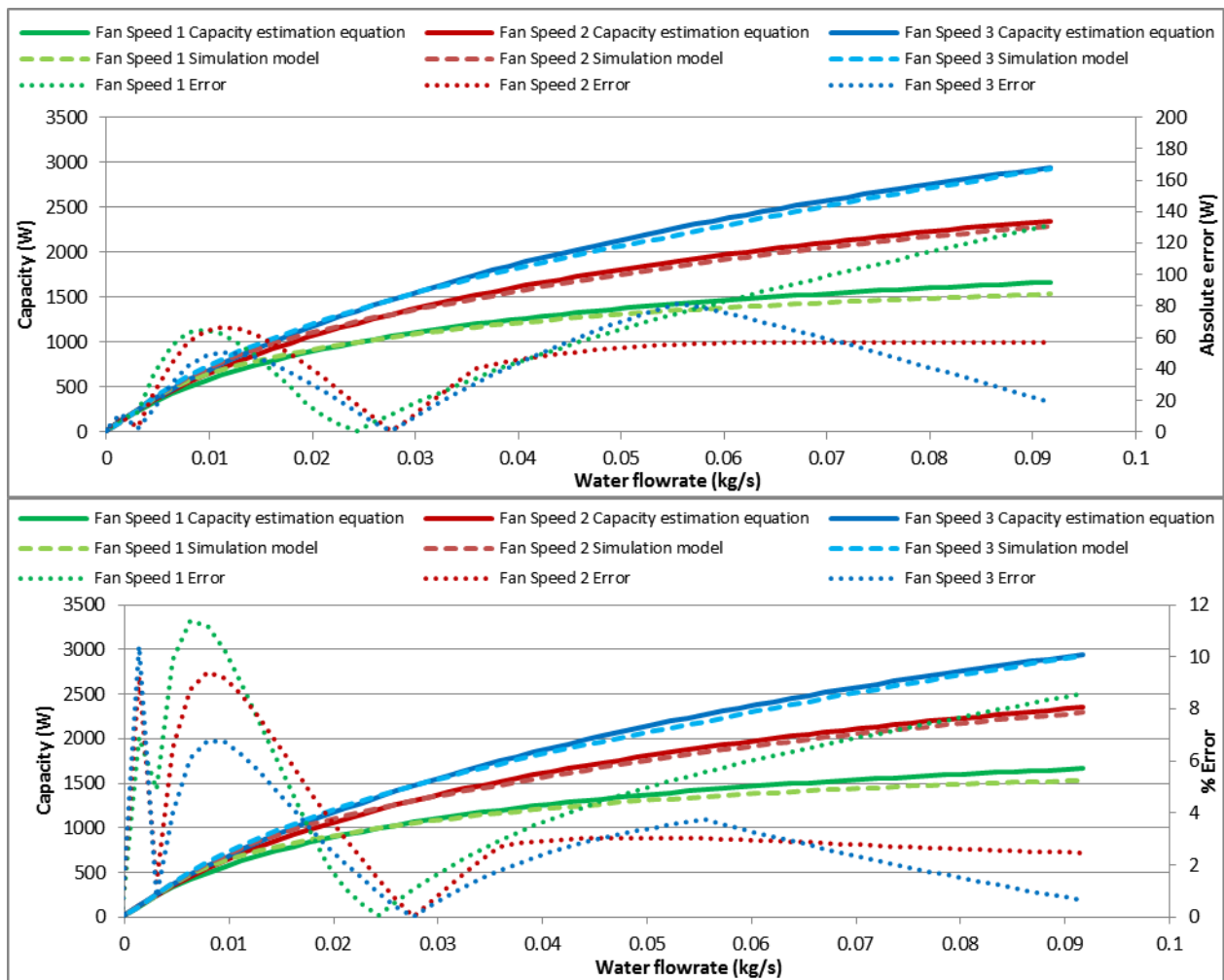
Figure 2: Water flow rate vs fan coil capacity and absolute error (control and simulation model)
