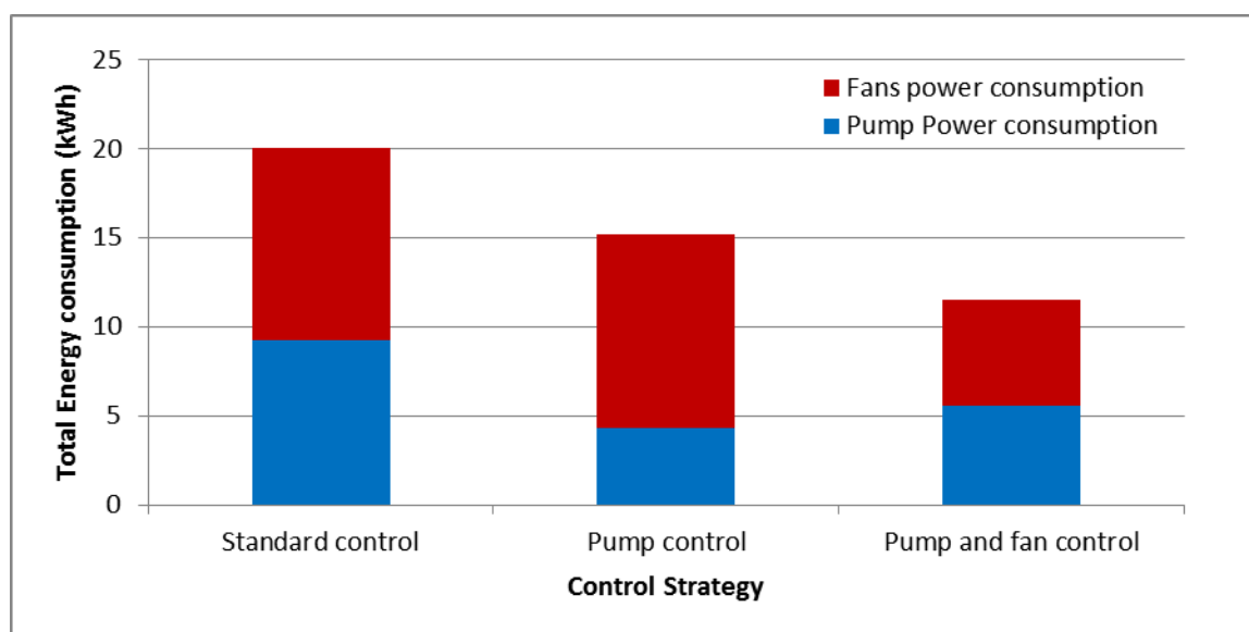
Figure 6: Fan and pump power consumption 7am – 9 pm for the three control strategies
