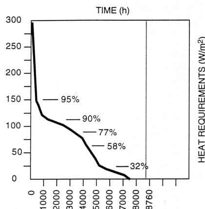
Percentual coverage of annual heat demand for greenhouse heating by alternative energy sources relative to Naaldwijk, Netherlands (from van den Braak and Knies, 1985)
