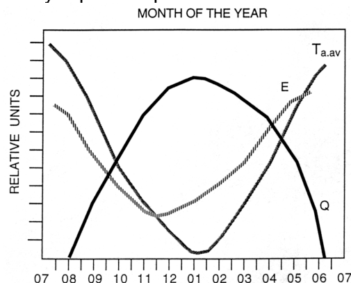
Heat requirement fluctuations in a greenhouse over a typical year in Gevgelija, Republic of Macedonia (from Popovski, 1984). E = solar radiation energy flux ( \text{Wh/m}^2 ); T_{a.av} = monthly average outside air temperature ( ^{\circ}\text{C} ); Q = greenhouse heat requirements (W)
