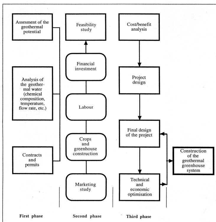
Fig.19. Block diagram of the development of a geothermal greenhouse heating project
