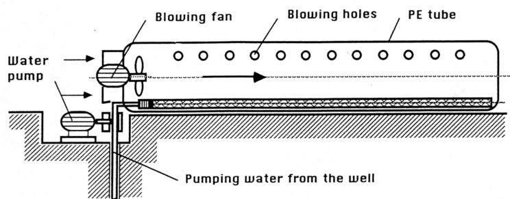
Fig.14. Water/air heat exchanger in air distribution tube (Grafiadellis, 1986)
