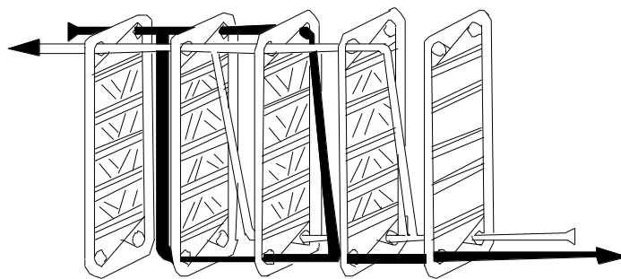
Fig.6. Plate heat exchanger
