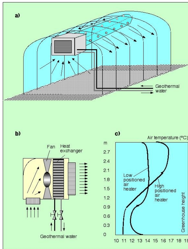
a) Position of the 'fan-jet' heating system in a greenhouse; b) layout of a fan-assisted convector unit; c) vertical temperature profiles in a greenhouse heated with fan convector units at different heights
