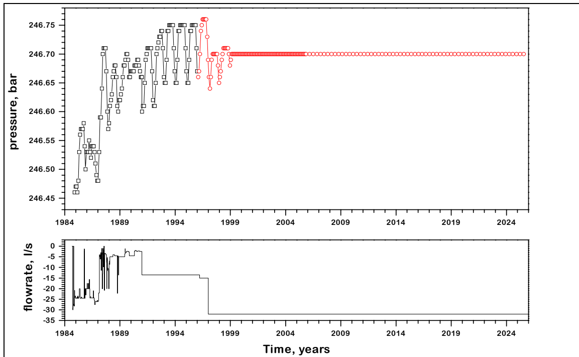
Figure 10: Simulated pressure / flowrate history for the producer block, losia doublet
