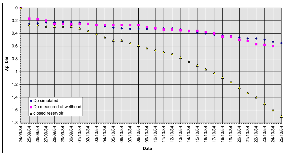
Figure 9: Calibration results, Well 4005 Oradea
