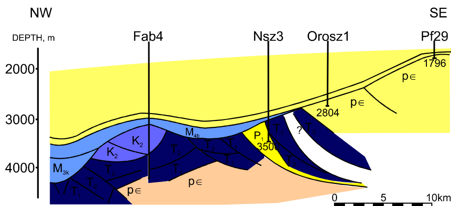
Figure 12: NW-SE Cross section through the Nagyszénás-Fabiánsebestyén area (source MOL Geothermal)
