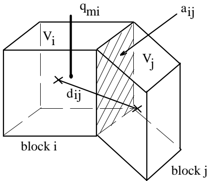
Figure 2: Block discretization
