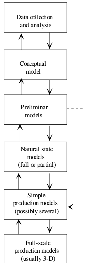
Figure 3: Modelling steps
