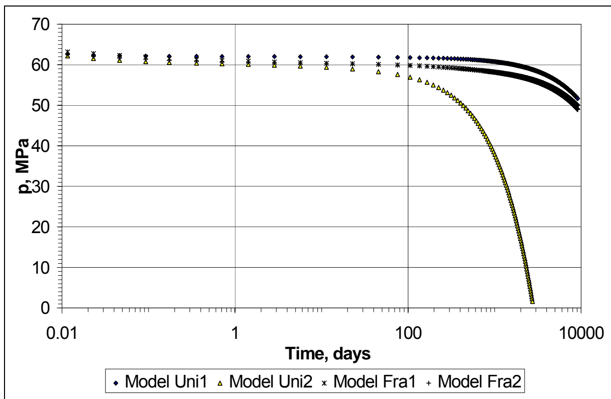
Figure 16: 1MW production simulation semilog plot
