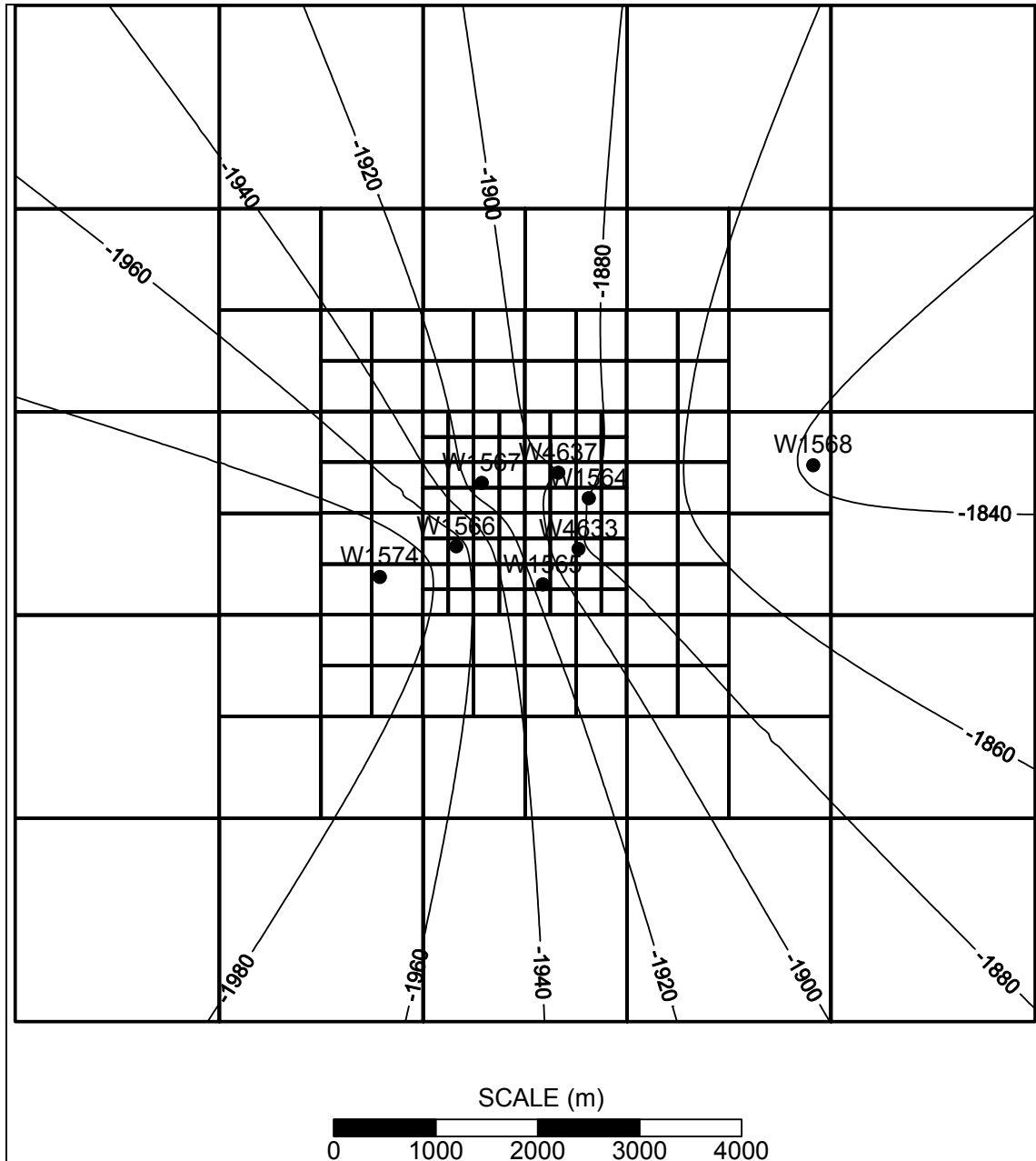
Figure 4: Simulation grid set-up and contour lines at the top of Upper Pannonian
