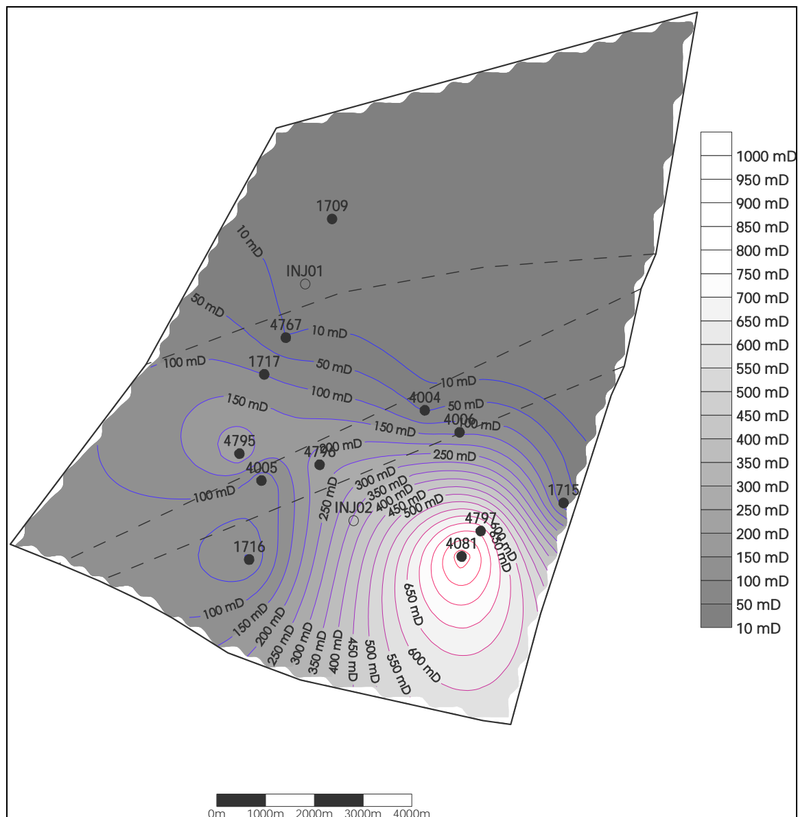
Figure 7: Permeability distribution of the Oradea reservoir model
