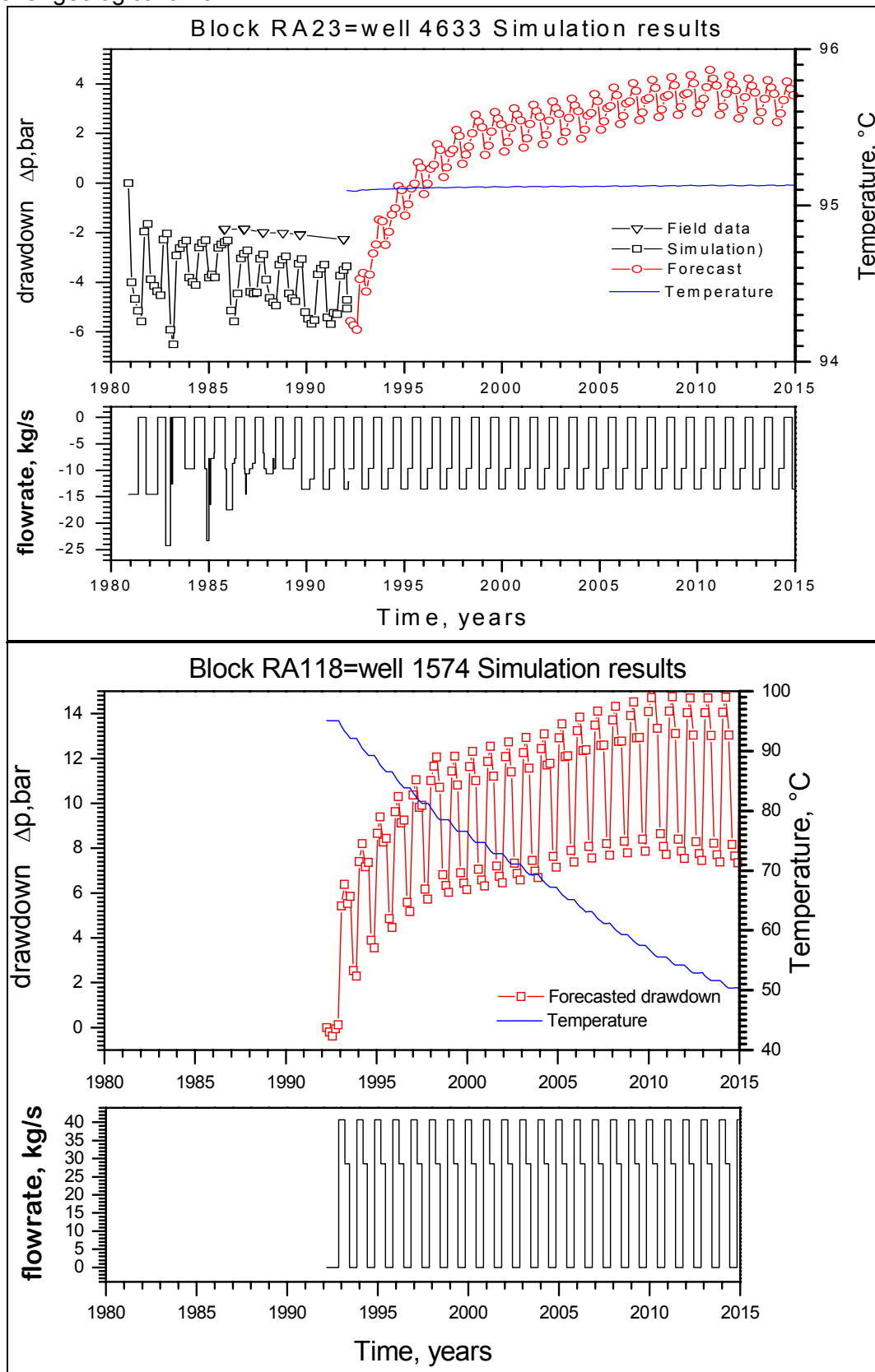
Figure 5: Tomnatic reservoir simulation results
