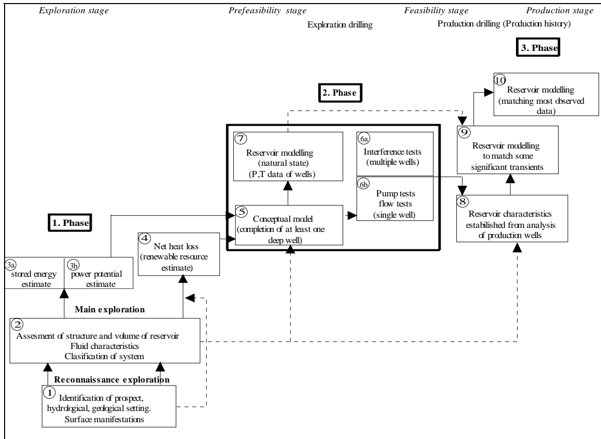
Figure 1: Schematic flow diagram showing reservoir assessments at various stages of the development of a geothermal project
