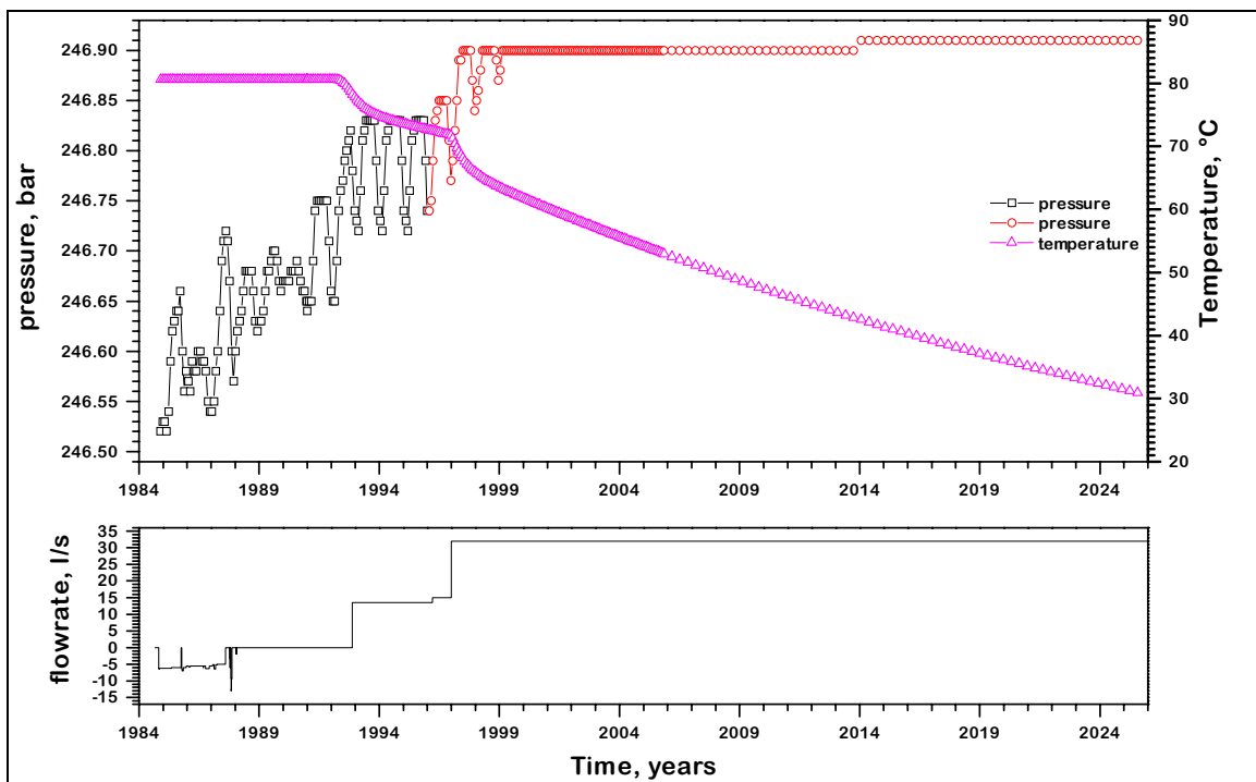
Figure 11: Simulated pressure / temperature / flowrate history for the injector block, losia doublet
