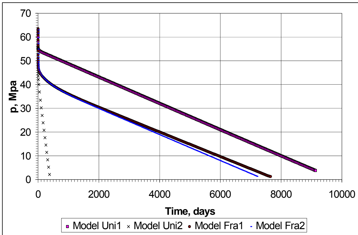
Figure 17: 5MW production simulation
