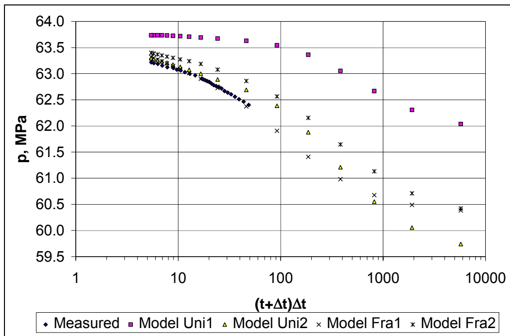
Figure 14: Horner plot of measured and simulated build-up
