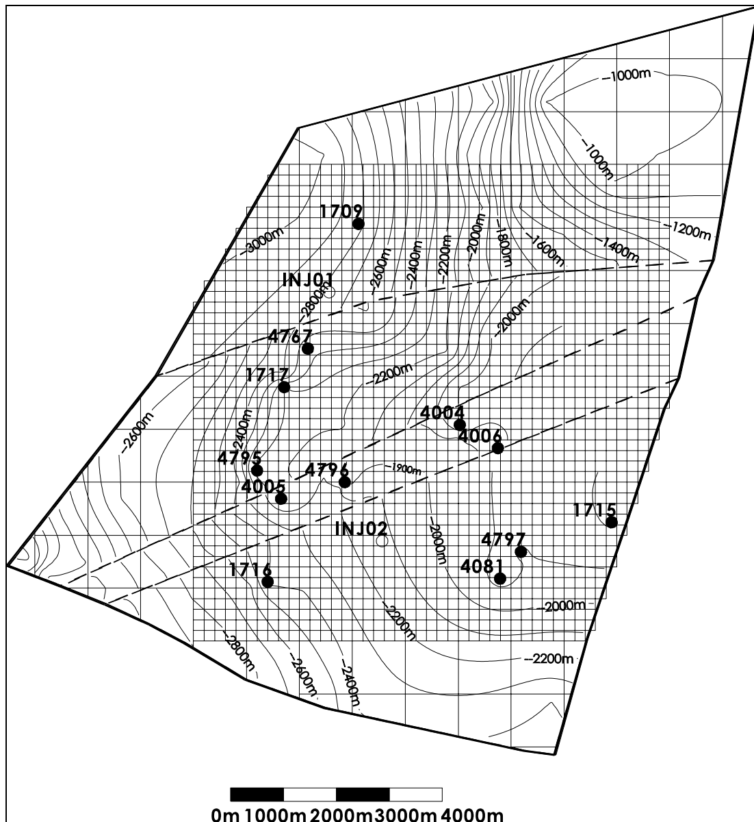
Figure 6: Oradea reservoir simulation. Grid set-up and contour map at the top of the reservoir
