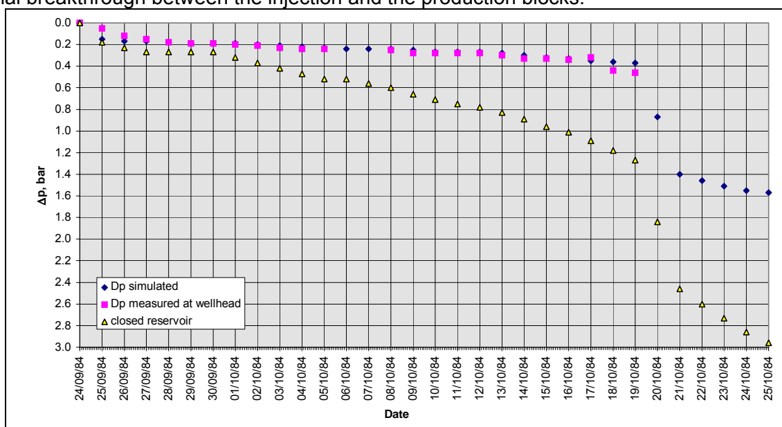
Figure 8: Calibration results, Well 4004 Oradea
