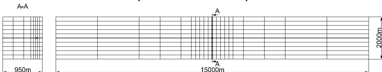
Figure 13: Grid set-up
