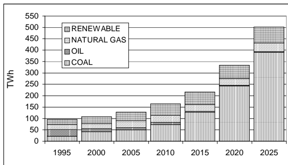
Figure-3 Projection of Electricity Supply by Fuel Mix (Including PLN, IPPs and Captive Power)
