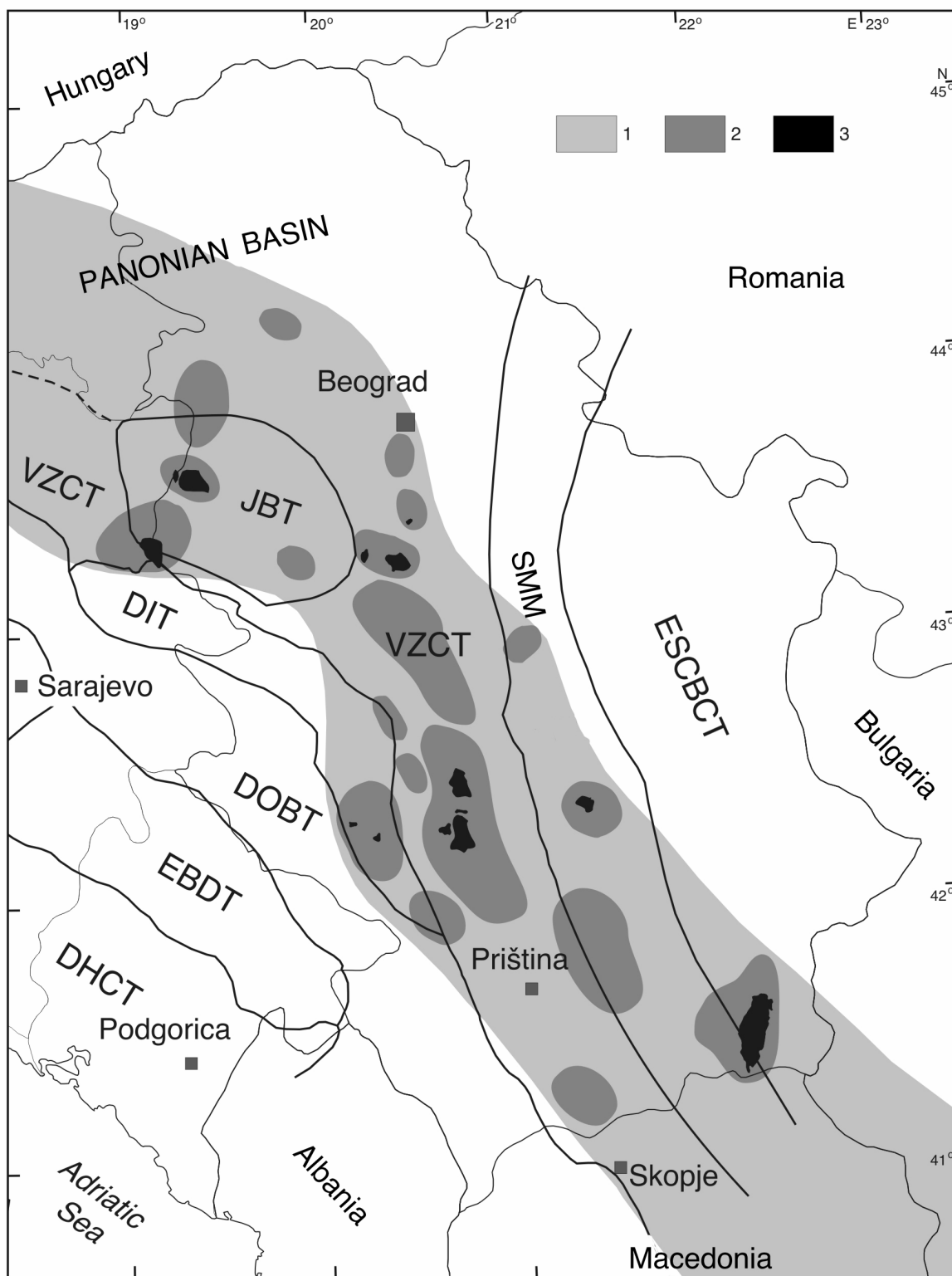
Figure 1. Locations of magmatic rocks occurrences of neogene age at the territory of Serbia (explanation in text for geotectonic units-terranes), (1-zone with occurrences of volcanic rocks; 2-granitoid pluton; 3-granitoid at the surface).
