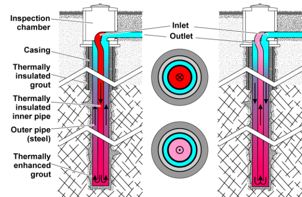
Figure 1: Schematic horizontal and vertical cross sections of a deep coaxial borehole heat exchanger used as heat storage in summer (charge of the storage as CXC flow, left side and upper middle) and winter (discharge of the storage as CXA flow, right side and lower middle), respectively. Note that only the crystalline bedrock is used as heat storage while the caprock including possible aquifers are thermally insulated.
