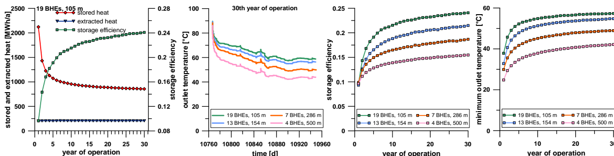
Figure 6: (From left to right): Stored heat, extracted heat and storage efficiencies of the set up with 19 BHEs; comparison of the outlet temperatures in the 30th year of operation and of the storage efficiencies and minimum outlet temperatures (right) for the four different preliminary set ups.
