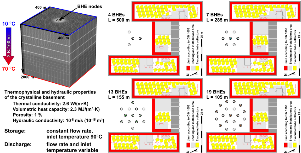
Figure 5: (left): General set up, parameters, boundary conditions and flow rates and temperature during storage and extraction of the numerical FEFLOW models. (right): Layout of the BHEs in top view of the modelled office building including the position of the evacuated tube collectors installed on the building's roof for the four different preliminary set ups: 4, 7, 13 and 19 BHE's with the same total BHE length for the BTES.
