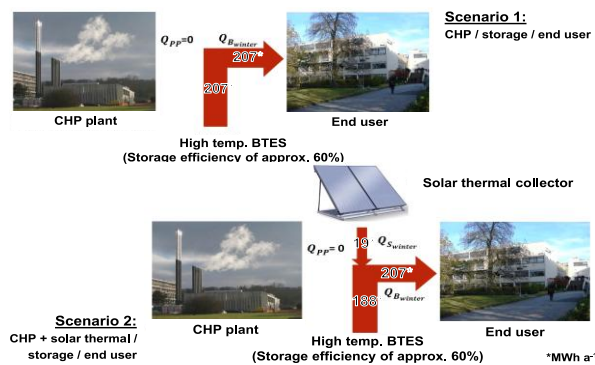
Figure 4: Winter operation modes for scenarios (1) and (2) respectively with coupling of combined heat and power (CHP) plant, solar thermal collectors and MH-BTES. Numbers are annual heat flows in MWh assuming a storage efficiency of 60%.
