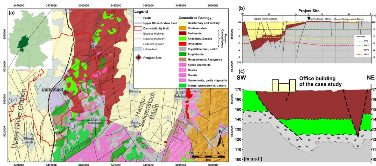
Figure 2: (a) Simplified geological map of the project site at the eastern Upper Rhine Graben fault, after [13]. (b) Schematic W-E-cross section of the northern Upper Rhine Graben and accompanying graben shoulders including major isotherms [14]. (c) Schematic SW-NE-cross section of the project site, modified from [11], symbol w indicates weathered zone at the top of the crystalline bedrock.
