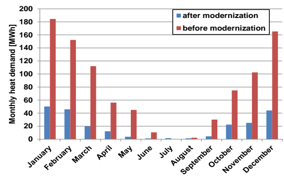
Figure 5: Comparison of the modelled monthly heat demand of the project building before and after the modernization in 2012.
