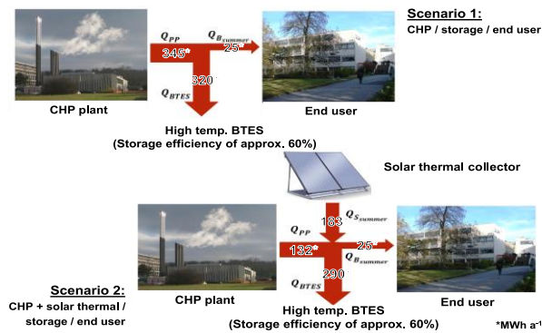
Figure 3: (top): summer operation mode of scenario 1 with the combined heat and power (CHP) plant covering both the heat demand of the building and the MD-BTES. (bottom): summer operation mode of scenario 2 with the coupling of the CHP and solar thermal collectors to cover the heat demand of the building and the MD-BTES. Numbers are annual heat flows in MWh assuming a storage efficiency of 60%.
