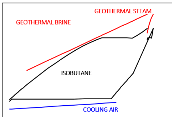
Figure 4 - (T, Q) diagrams for one pressure level and two pressure level cycle
