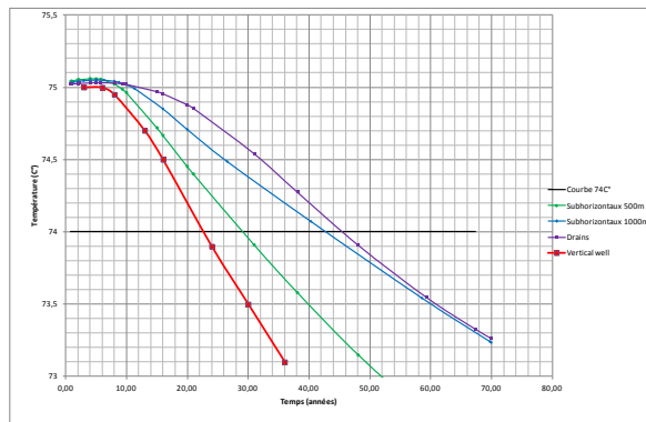
Figure 7: Impacts on cooling kinetics. A selected well/drain designs
