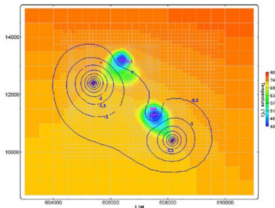
Figure 11 : Temperature and pressure drawdown fields. Year 2044. 1 st reservoir layer. Conventional doublets scenario
