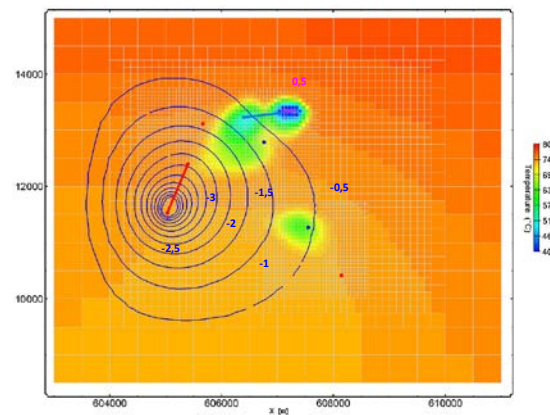
Figure 13 : Temperature and pressure drawdown fields. Year 2044. 2 nd reservoir layer. Sub-horizontal drain scenario
