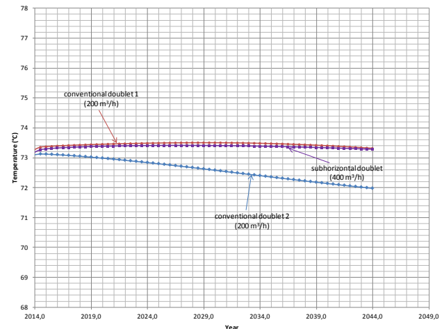
Figure 14: Cooling kinetics. Case study 2.
