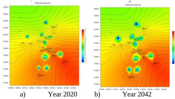
Figure 10: Reservoir simulation. Case history 2. Completed pressure and temperature fields. Sub-horizontal well scenario
