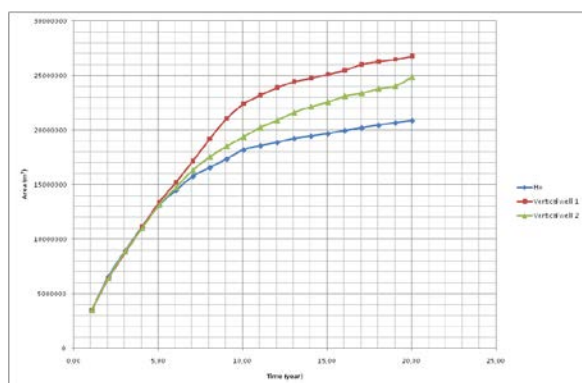
Figure 3: Cooling kinetics. Cold areal extents
