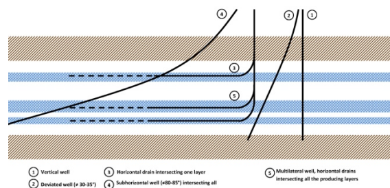
Figure 6: Candidate well/drain trajectories. Multilayered reservoir
