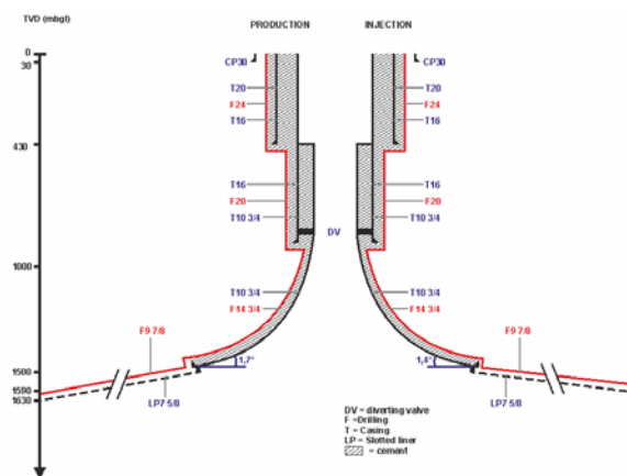
Figure 9: GDH doublet (sub) horizontal well profiles
