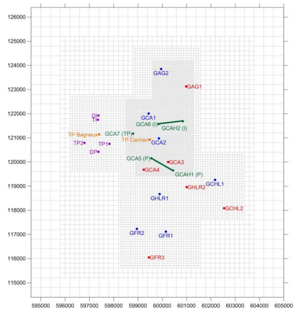
Figure 8: Reservoir simulation grid and well (existing, projected) locations (top reservoir impacts)
