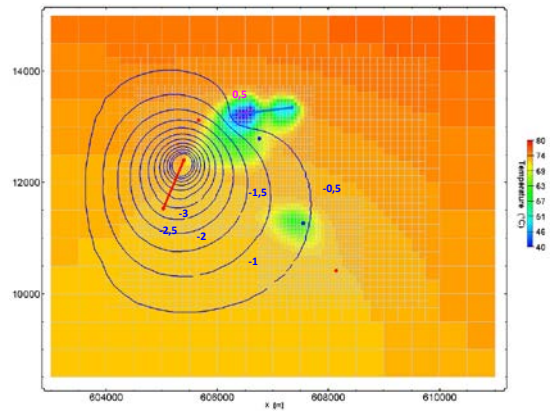
Figure 12 : Temperature and pressure drawdown fields. Year 2044. 1 st reservoir layer. Sub-horizontal drain scenario
