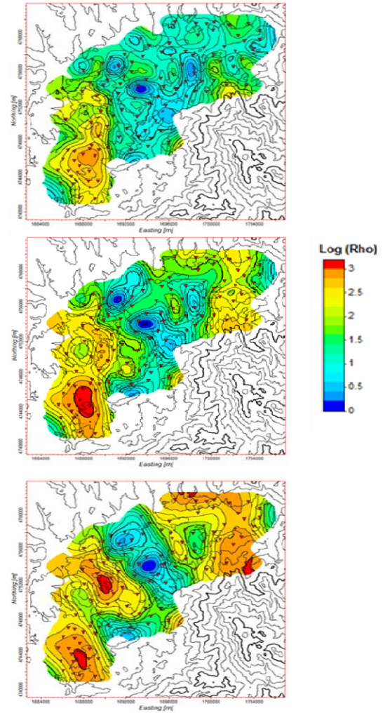
Figure 6: Resistivity maps at different depths for the Cinigiano-Montalcino area: 1000m (top panel), 1500m (middle panel), 2000m (bottom panel)
