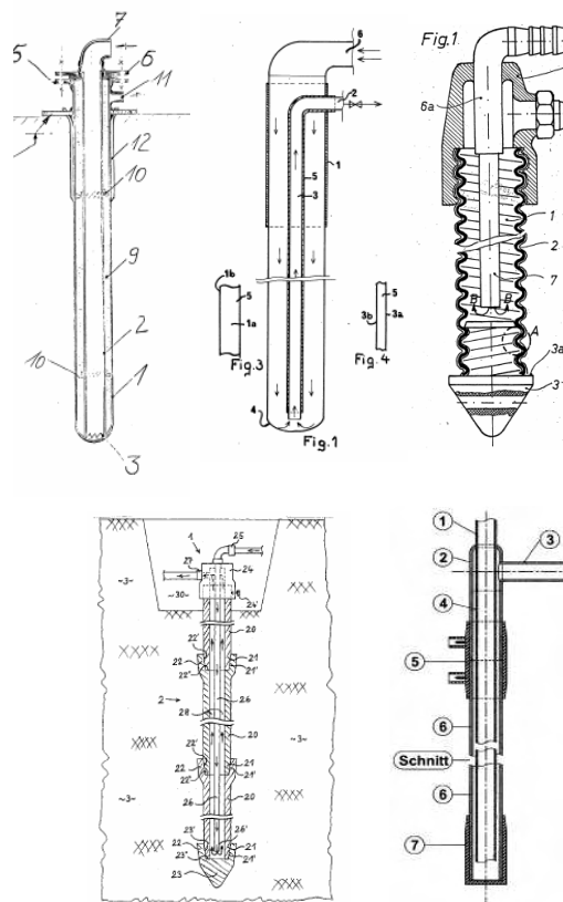
Figure 2: Examples of drawings of coaxial BHE from German Patent applications, upper row from left: Brocks & Richter (1980), Hinterding (1981), Hund (1983); lower row from left: Waterkotte (2003), Rosinski (2006)
