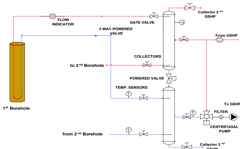
Figure 11: Installation schematic of BHE connection to heat pumps in EST mechanical engineering building
