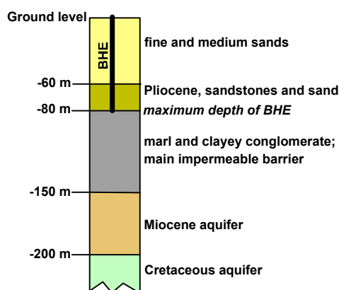
Figure 10: Geological underground situation at EST mechanical engineering building site
