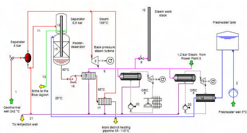
Figure 2: Flow diagram of the Svartsengi Power Plant.
