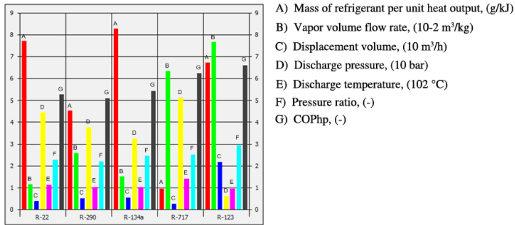
Fig. 4 The results for the selected refrigerants.
