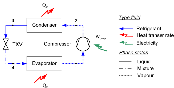
Fig. 3 A concept of a vapor compression heat pump for upgrading low temperature heat.
