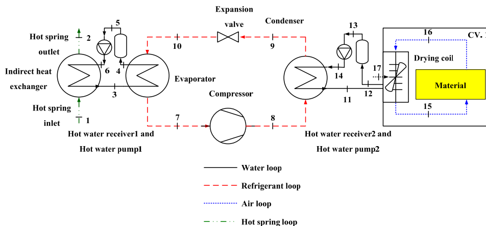
Fig. 5 Single diagram geothermal heat pump.
