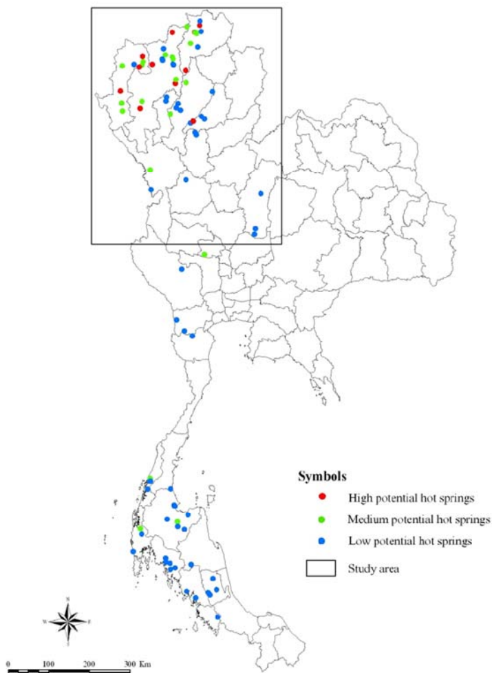
Fig. 1 Location map of hot springs in Thailand (CMU, 2008).
