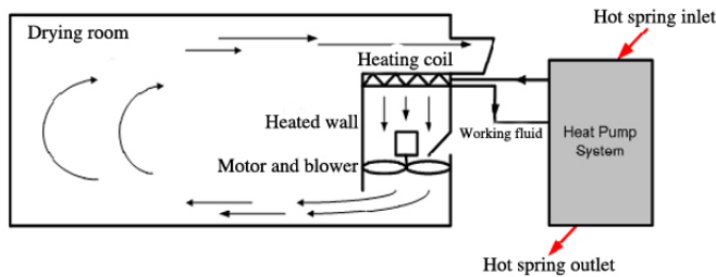
Fig. 6 Working steps of drying room with heat pump system.
