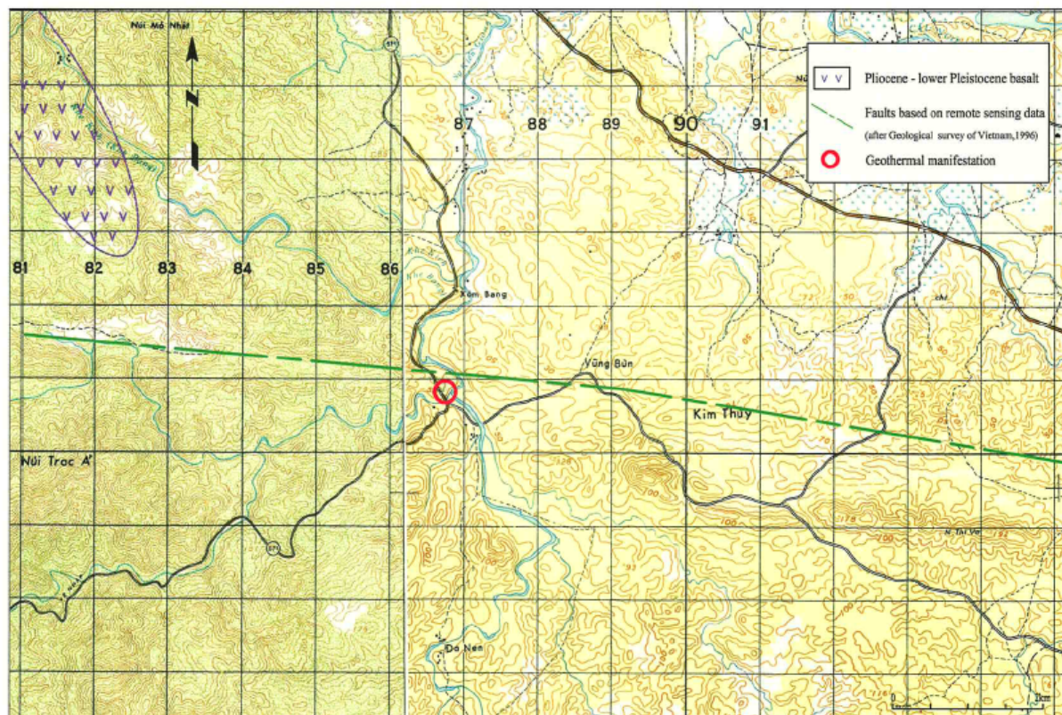
Figure1: Red circle is the location of Bang geothermal resource, will be intended to explore (according to data of J-Power).
