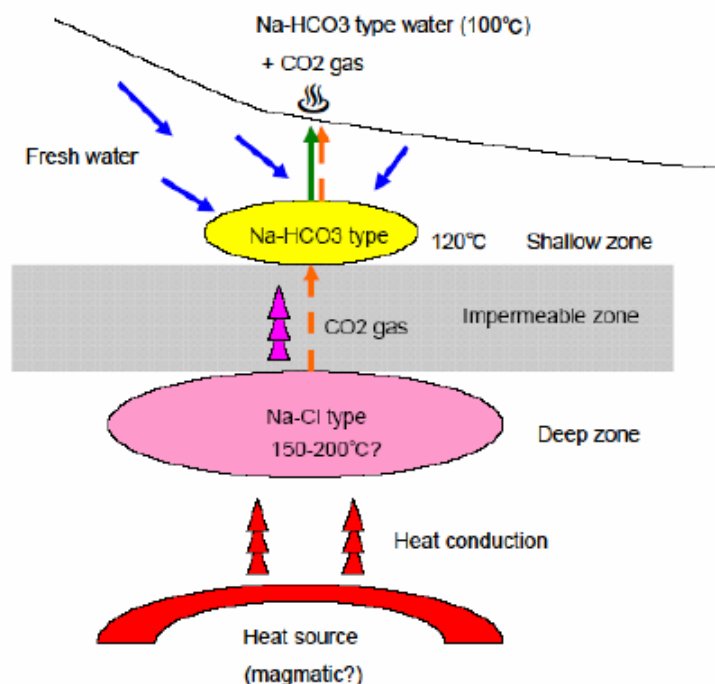
Figure 2: The geochemical modeling of Bang geothermal resource (according to data of J-Power).
