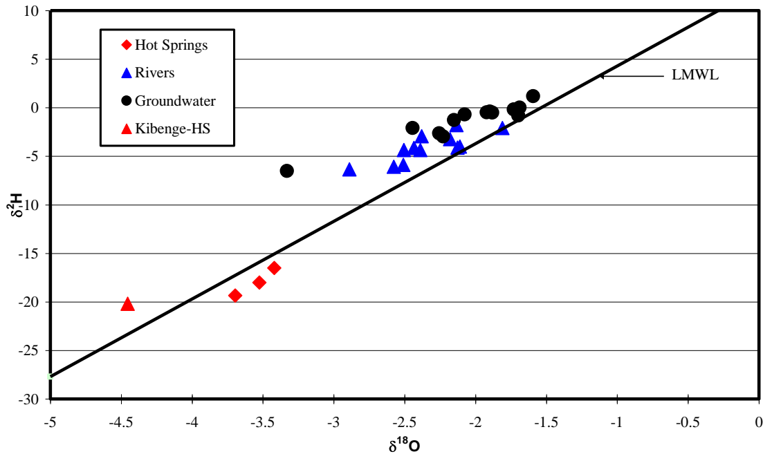
Figure 7: Buranga: stable isotopic composition of hot and cold water samples
