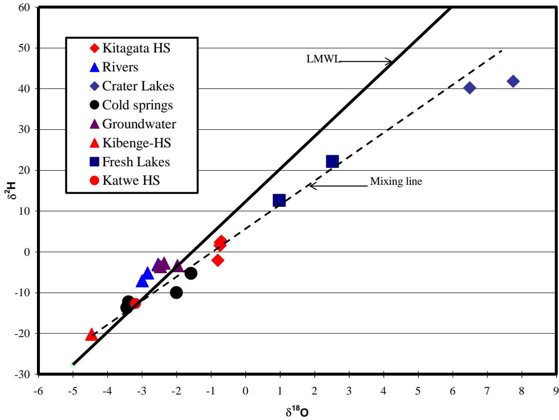
Figure 6: Katwe: stable isotopic composition of hot and cold water samples
