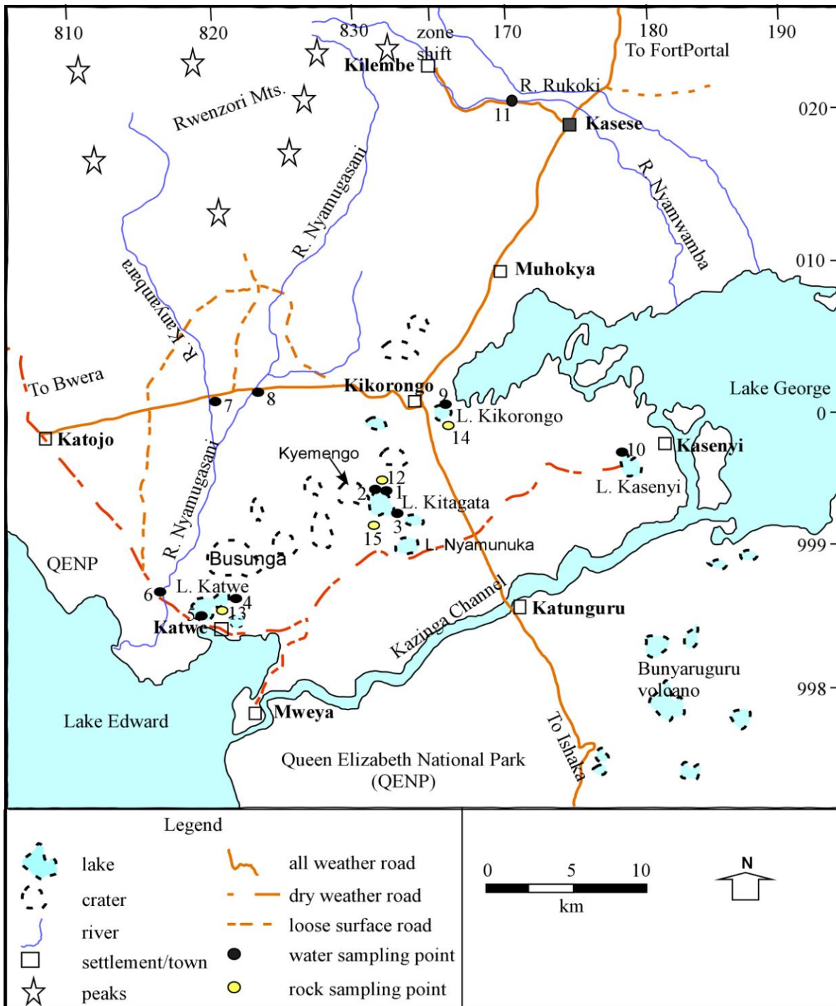
Figure 2: Katwe and surroundings. Geothermal, surface and ground water sampling points.
