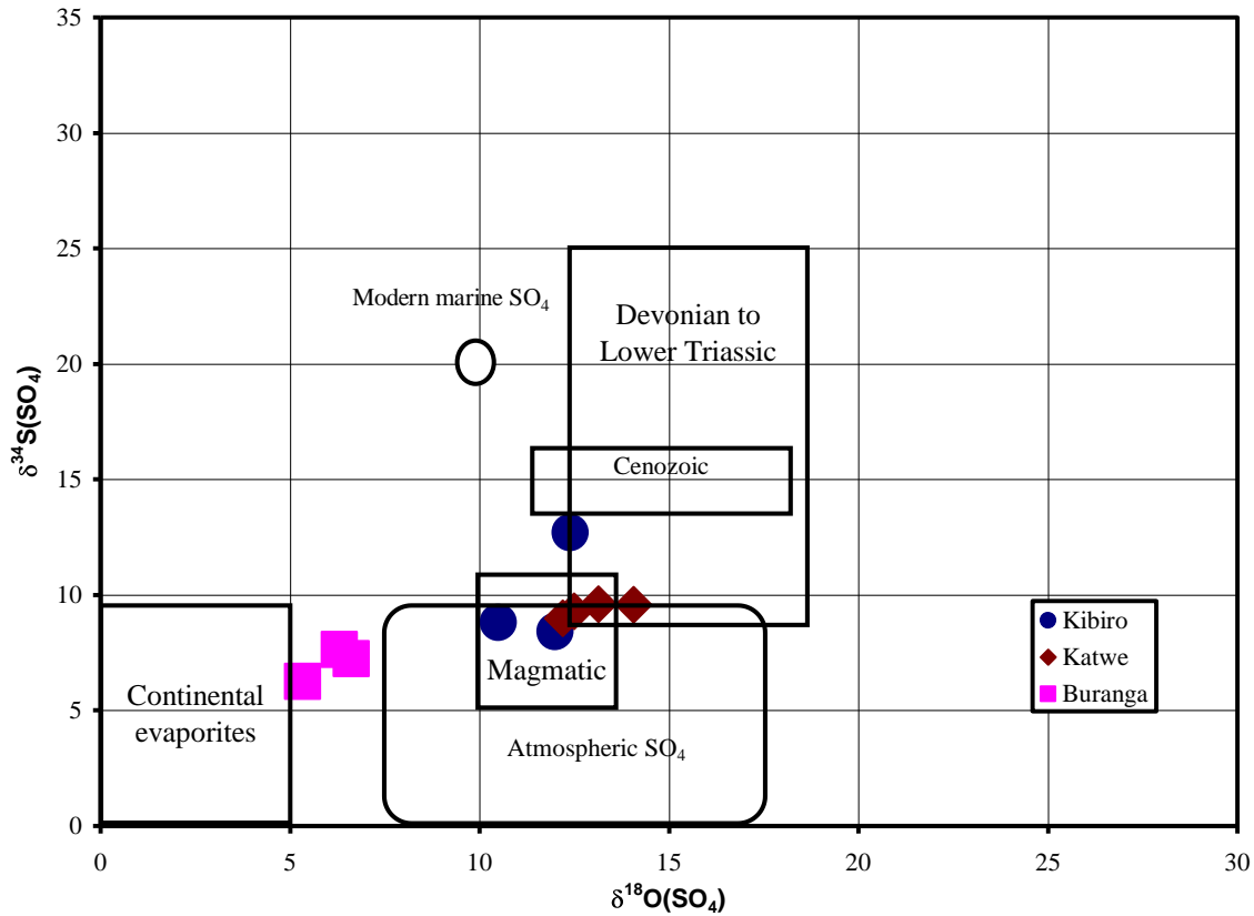
Figure 9: Katwe, Buranga and Kibiro: ranges of \delta^{34}\text{S} and \delta^{18}\text{O} of sulphates of various origins in groundwater
