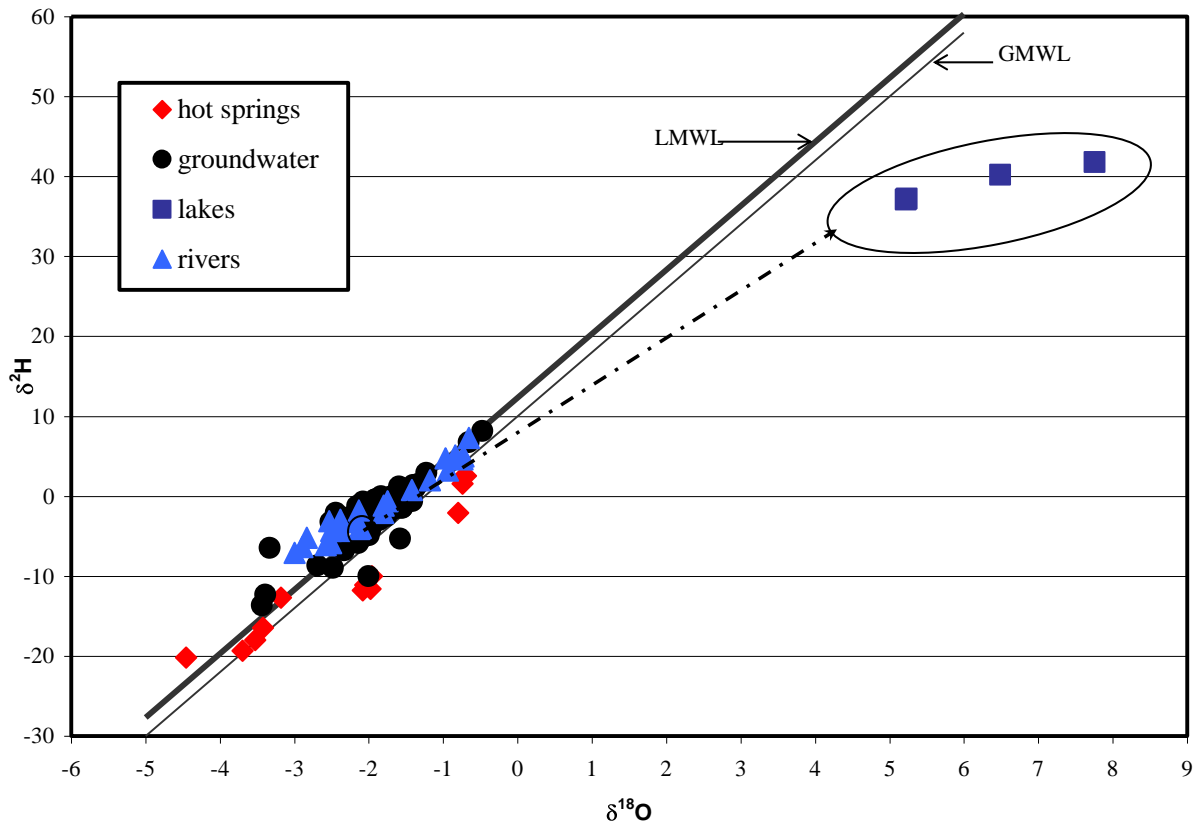
Figure 5: Katwe, Buranga and Kibiro: stable isotopic composition of hot and cold water samples.
