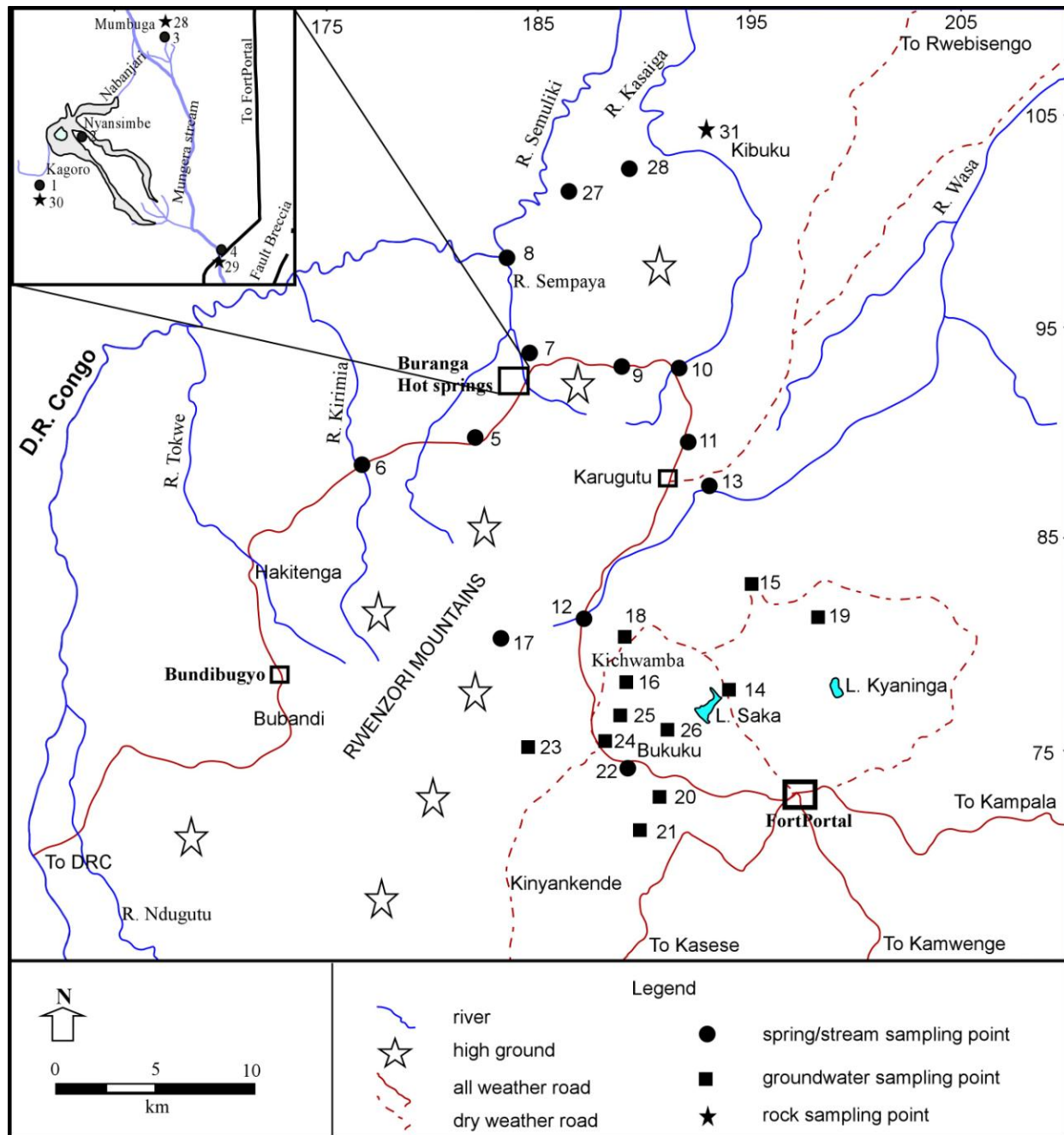
Figure 3: Buranga: geothermal, surface and ground water and rock sampling points.
