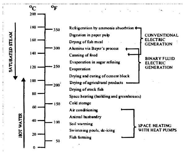
Figure 3. Lindal diagram.
