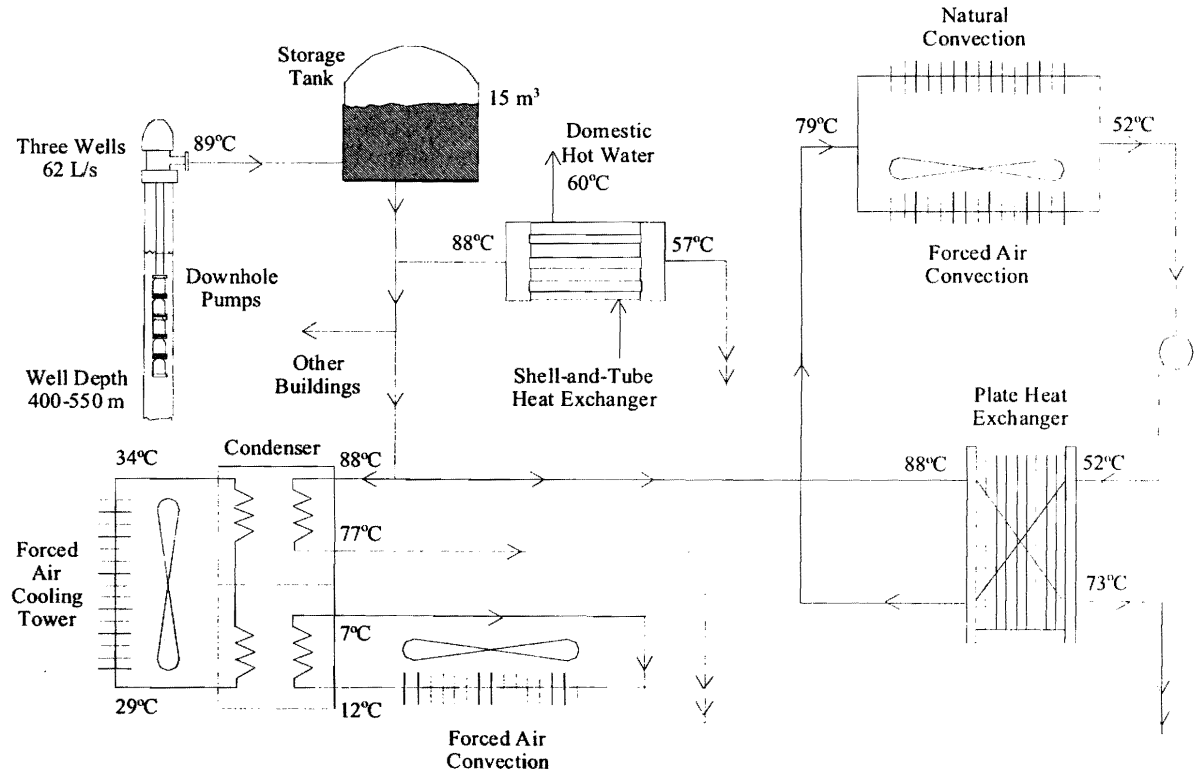
Figure 4. Oregon Institute of Technology heating and cooling system.
