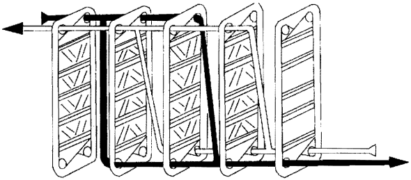
Figure 14. Plate heat exchanger.
