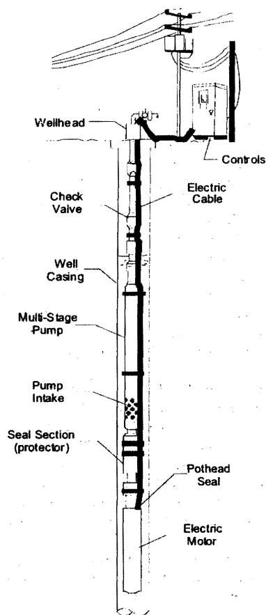
Figure 11. Submersible pump.
