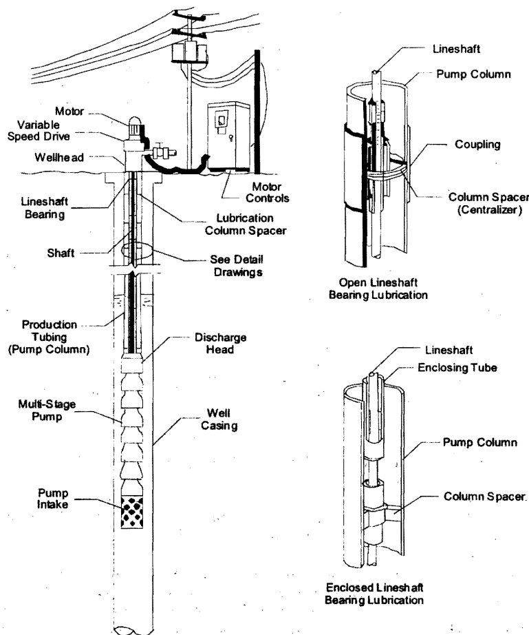
Figure 10. Lineshaft pump.
