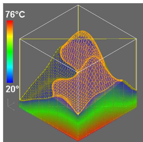
Figure 3: Run 1, 3D temperature voxel (1 million nodes) imported to the synthetic geology model space in GeoModeller. Visual-cut off of the mesh was set to 20.5^\circ\text{C} to allow the topography wire-frame to be viewed (All airspace is otherwise 20^\circ\text{C} , obeying the surface boundary condition.)
